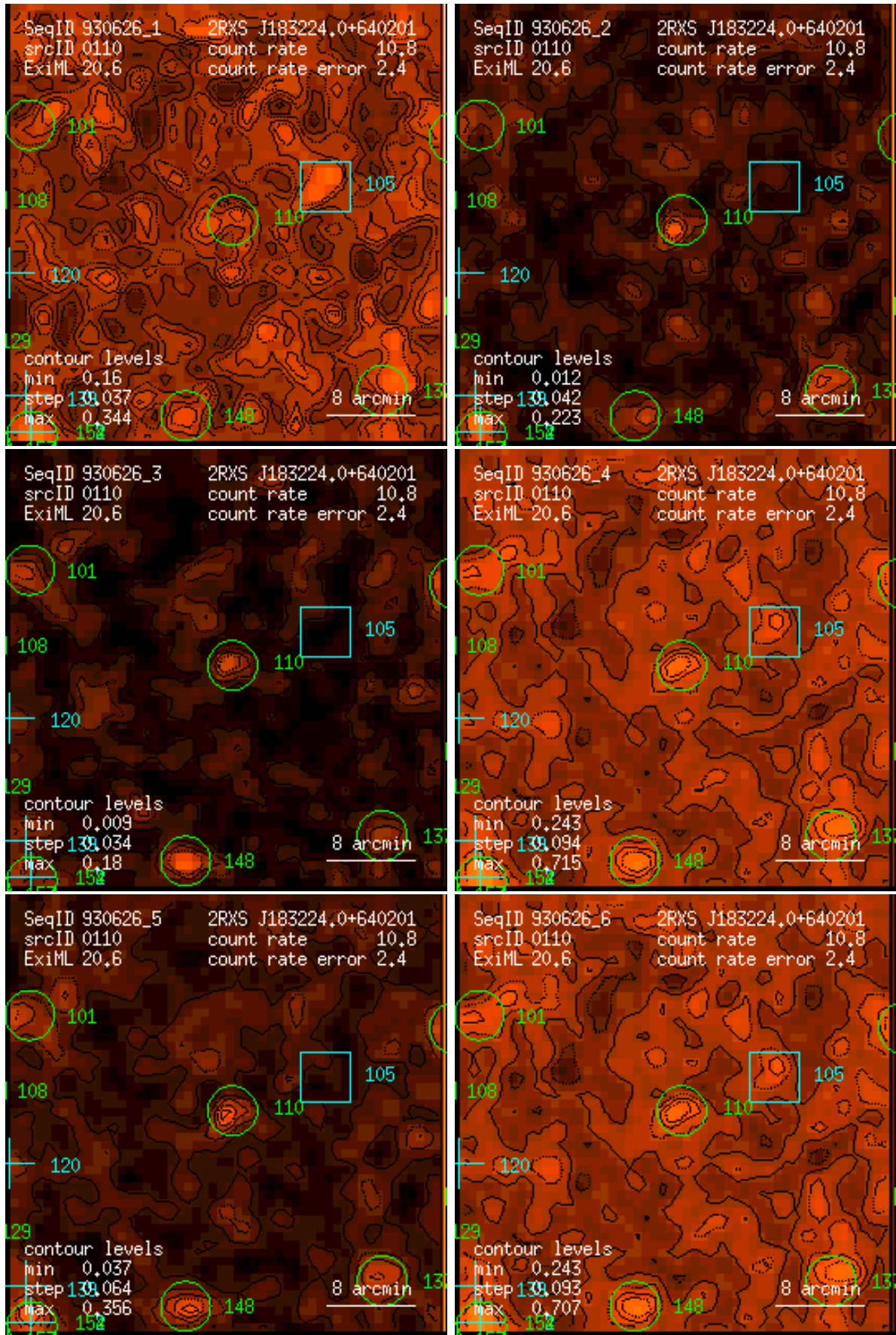
Figure 110: RASS 930626: detection 0110: band rate images, Gaussian filter: (1) PSPC channels 11 – 41, (2) 52 – 90, (3) 91 – 201, (4) 11 – 235, (5) 52 – 201, (6) 11 – 201. Broad band rates in counts/ks. Band rate contour levels in counts/ks/arcmin 2 .
