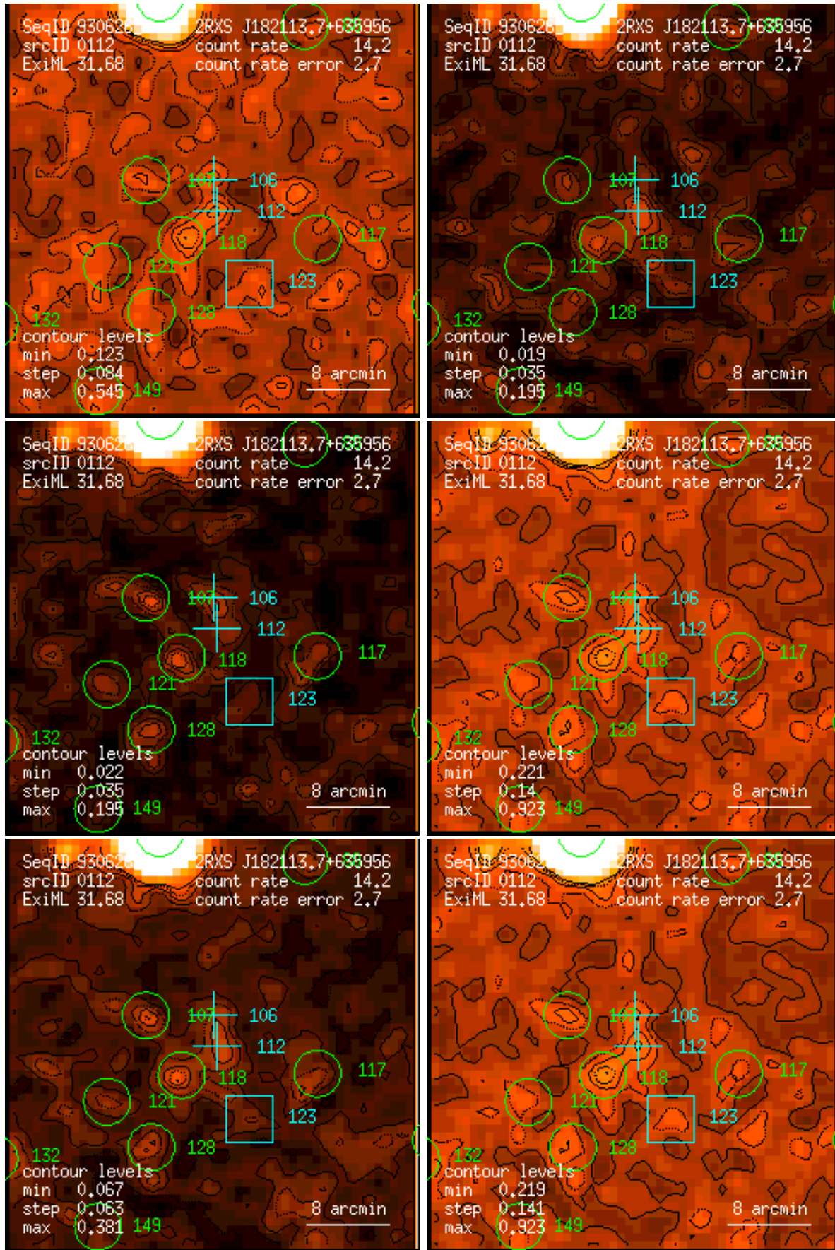
Figure 112: RASS 930626: detection 0112: band rate images, Gaussian filter: (1) PSPC channels 11 – 41, (2) 52 – 90, (3) 91 – 201, (4) 11 – 235, (5) 52 – 201, (6) 11 – 201. Broad band rates in counts/ks. Band rate contour levels in counts/ks/arcmin 2 .
