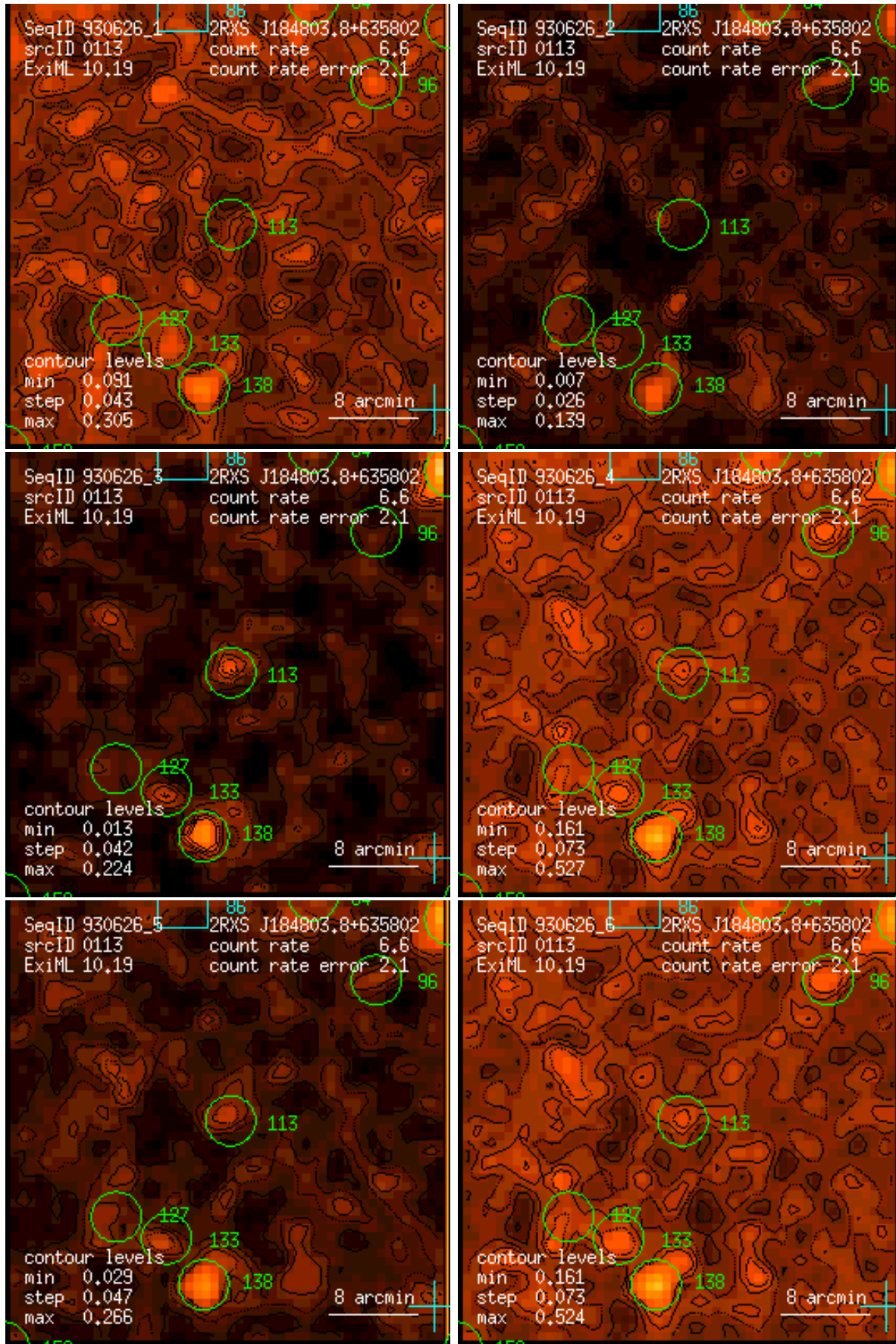
Figure 113: RASS 930626: detection 0113: band rate images, Gaussian filter: (1) PSPC channels 11 – 41, (2) 52 – 90, (3) 91 – 201, (4) 11 – 235, (5) 52 – 201, (6) 11 – 201. Broad band rates in counts/ks. Band rate contour levels in counts/ks/arcmin 2 .
