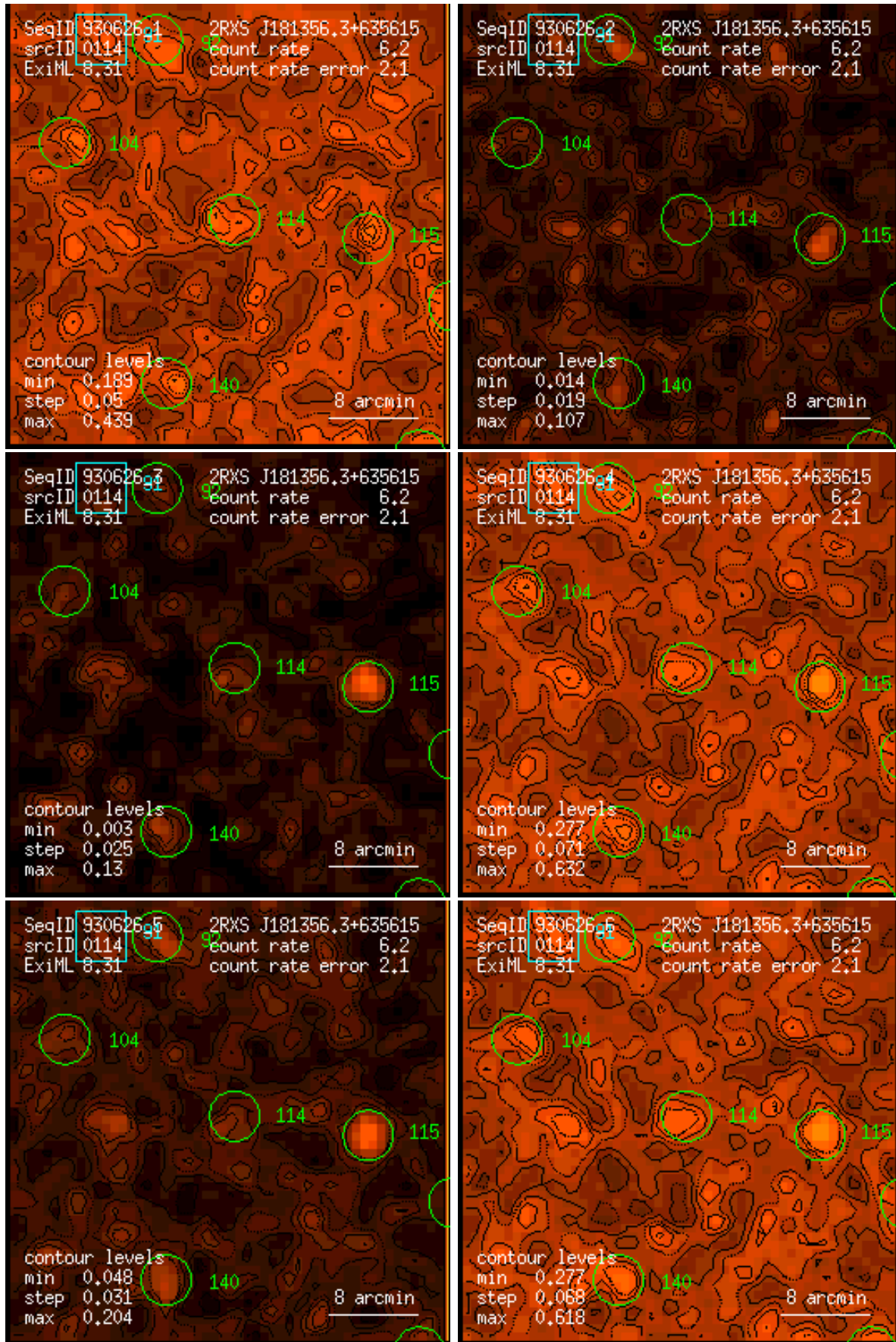
Figure 114: RASS 930626: detection 0114: band rate images, Gaussian filter: (1) PSPC channels 11 – 41, (2) 52 – 90, (3) 91 – 201, (4) 11 – 235, (5) 52 – 201, (6) 11 – 201. Broad band rates in counts/ks. Band rate contour levels in counts/ks/arcmin 2 .
