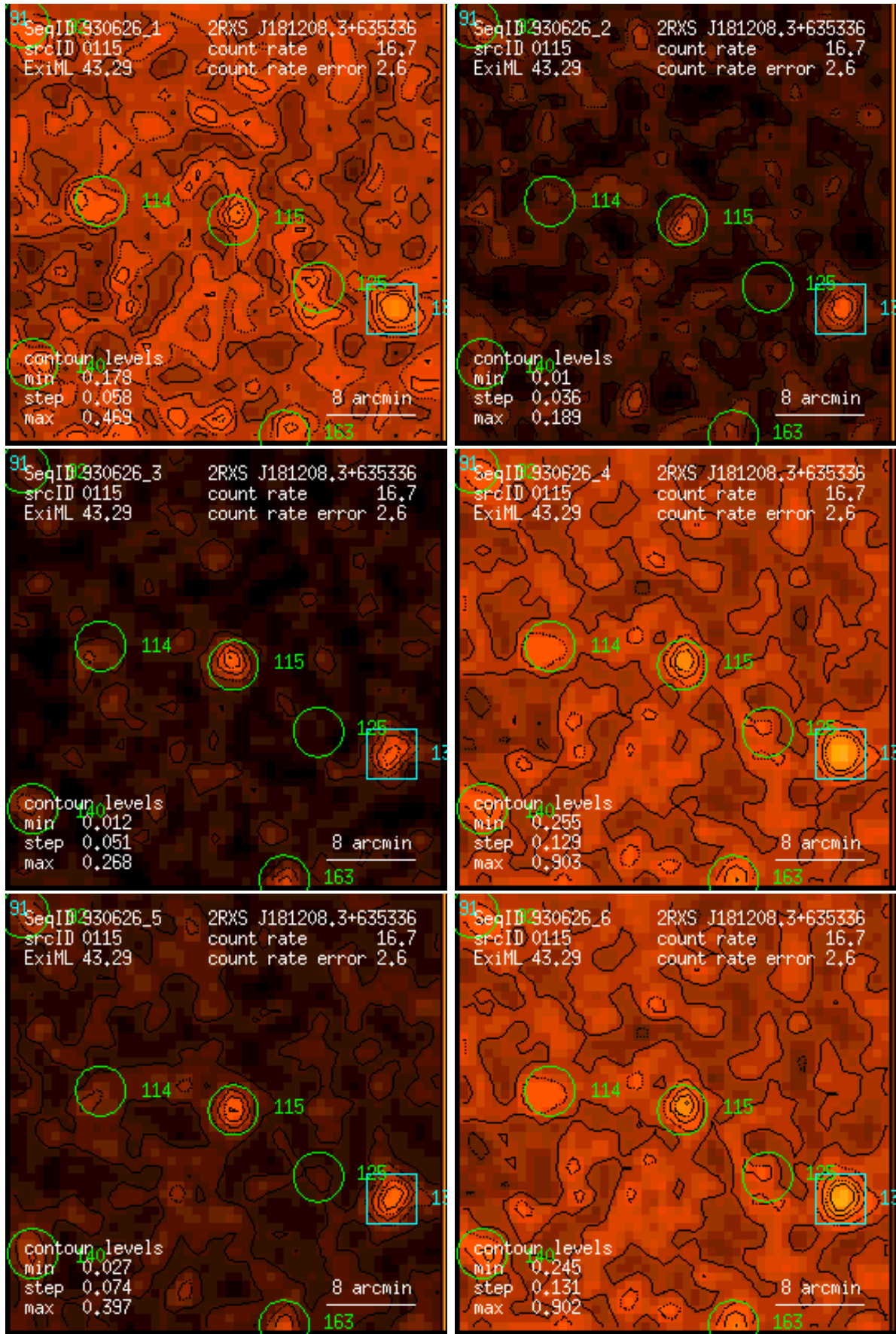
Figure 115: RASS 930626: detection 0115: band rate images, Gaussian filter: (1) PSPC channels 11 – 41, (2) 52 – 90, (3) 91 – 201, (4) 11 – 235, (5) 52 – 201, (6) 11 – 201. Broad band rates in counts/ks. Band rate contour levels in counts/ks/arcmin 2 .
