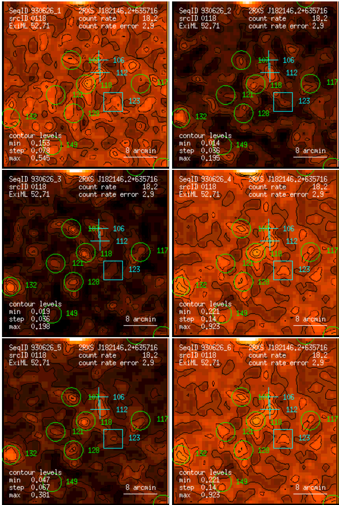
Figure 118: RASS 930626: detection 0118: band rate images, Gaussian filter: (1) PSPC channels 11 – 41, (2) 52 – 90, (3) 91 – 201, (4) 11 – 235, (5) 52 – 201, (6) 11 – 201. Broad band rates in counts/ks. Band rate contour levels in counts/ks/arcmin 2 .
