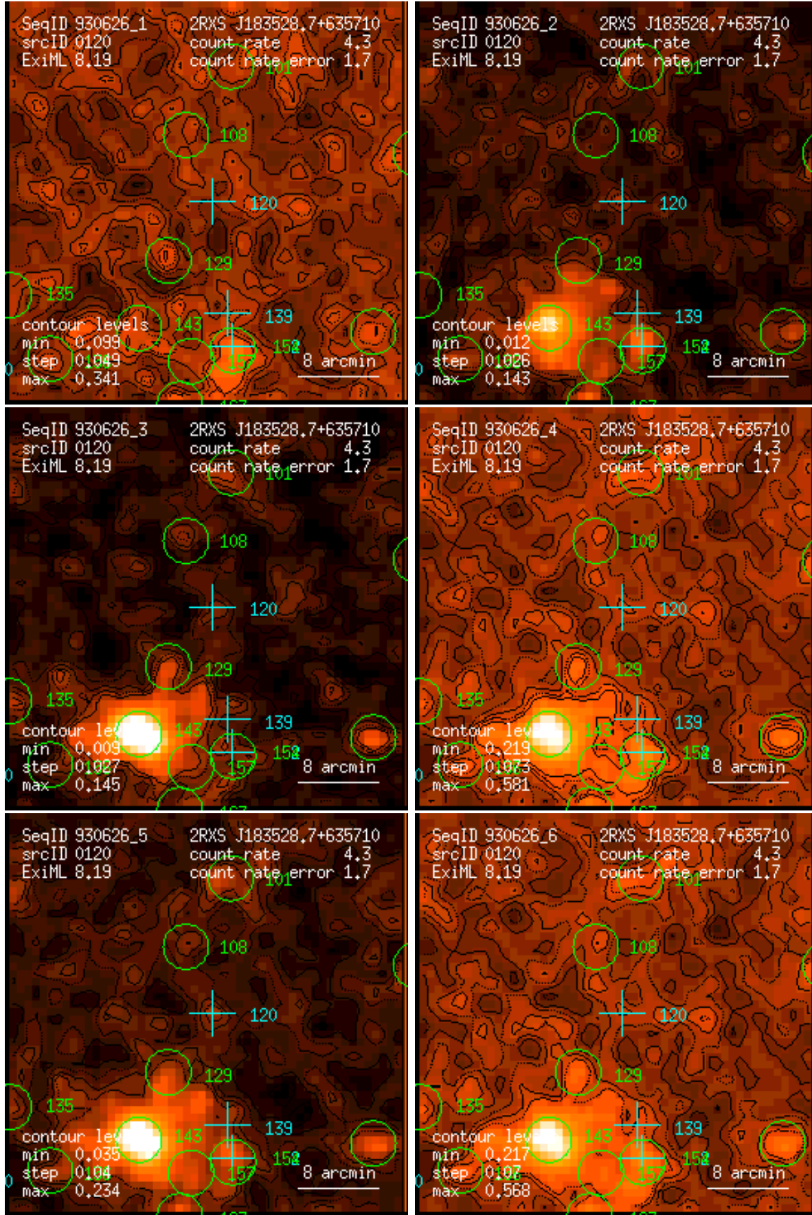
Figure 120: RASS 930626: detection 0120: band rate images, Gaussian filter: (1) PSPC channels 11 – 41, (2) 52 – 90, (3) 91 – 201, (4) 11 – 235, (5) 52 – 201, (6) 11 – 201. Broad band rates in counts/ks. Band rate contour levels in counts/ks/arcmin 2 .
