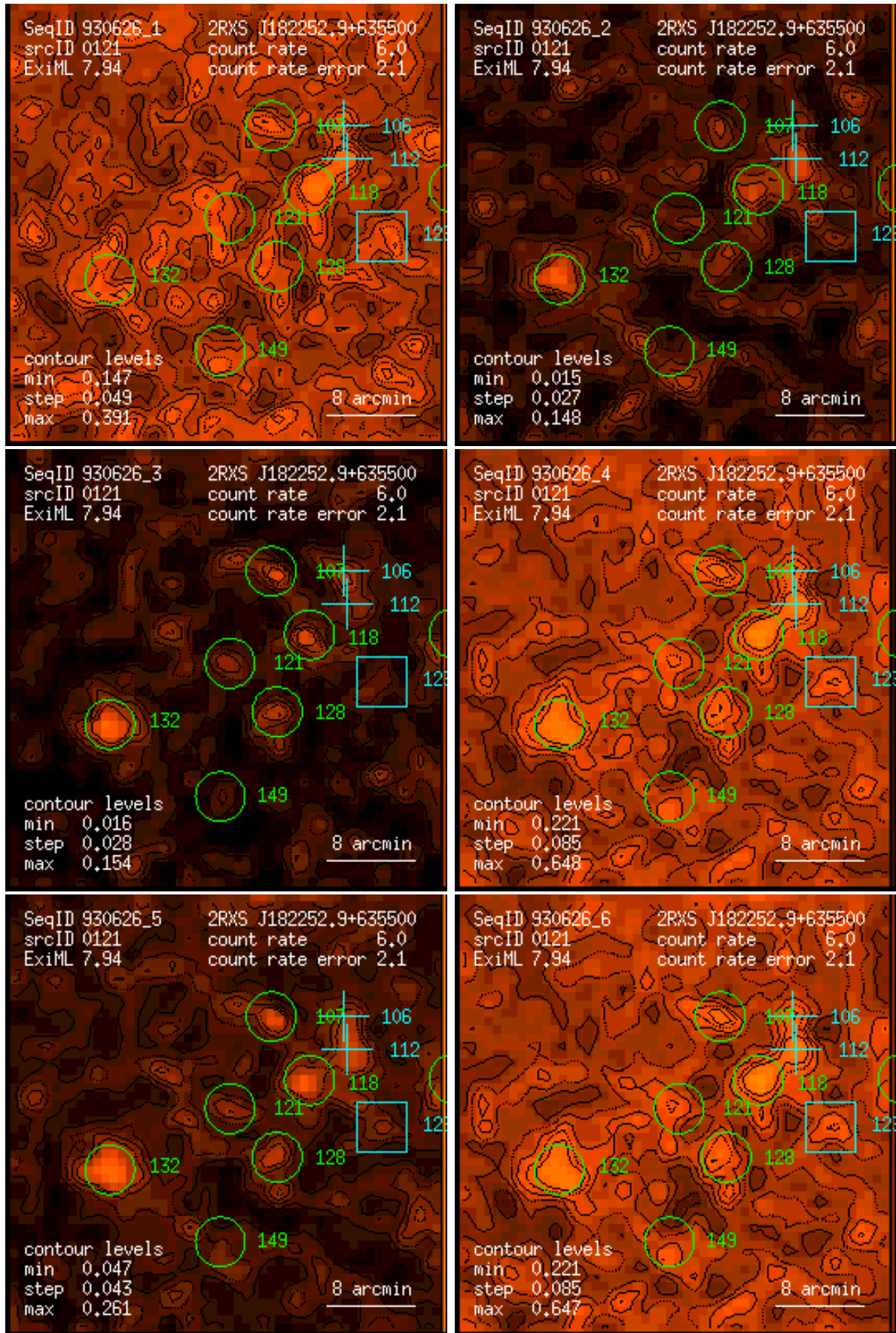
Figure 121: RASS 930626: detection 0121: band rate images, Gaussian filter: (1) PSPC channels 11 – 41, (2) 52 – 90, (3) 91 – 201, (4) 11 – 235, (5) 52 – 201, (6) 11 – 201. Broad band rates in counts/ks. Band rate contour levels in counts/ks/arcmin 2 .
