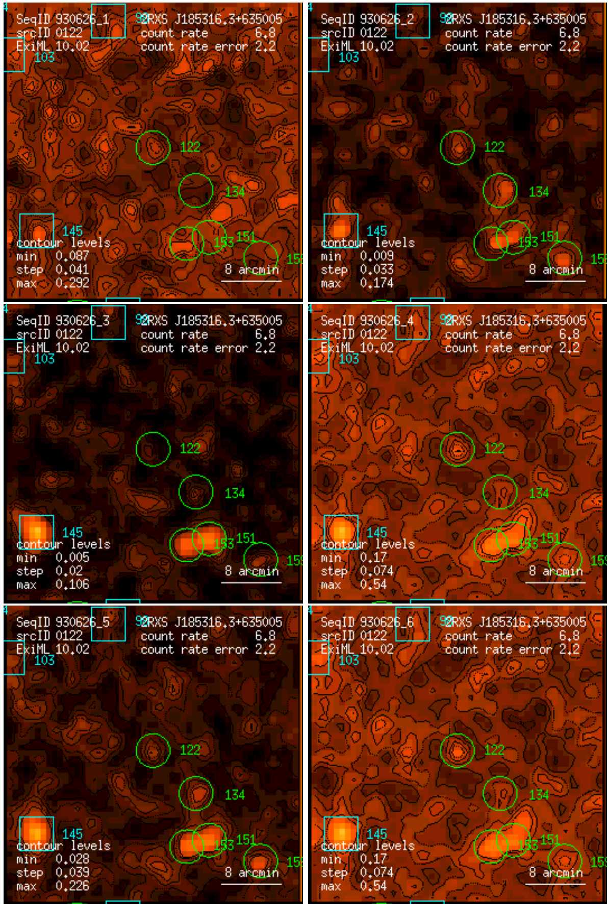
Figure 122: RASS 930626: detection 0122: band rate images, Gaussian filter: (1) PSPC channels 11 – 41, (2) 52 – 90, (3) 91 – 201, (4) 11 – 235, (5) 52 – 201, (6) 11 – 201. Broad band rates in counts/ks. Band rate contour levels in counts/ks/arcmin 2 .
