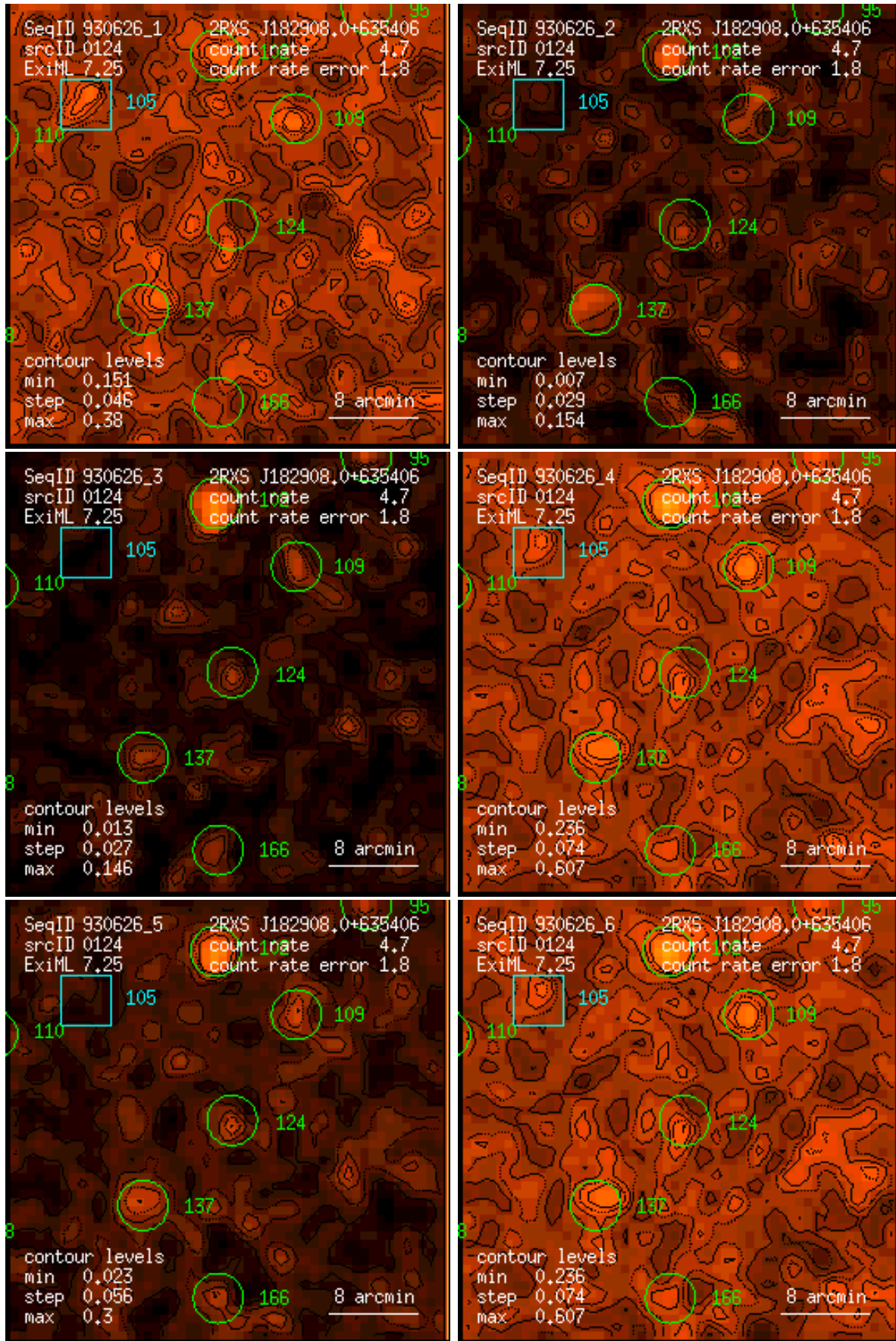
Figure 124: RASS 930626: detection 0124: band rate images, Gaussian filter: (1) PSPC channels 11 – 41, (2) 52 – 90, (3) 91 – 201, (4) 11 – 235, (5) 52 – 201, (6) 11 – 201. Broad band rates in counts/ks. Band rate contour levels in counts/ks/arcmin 2 .
