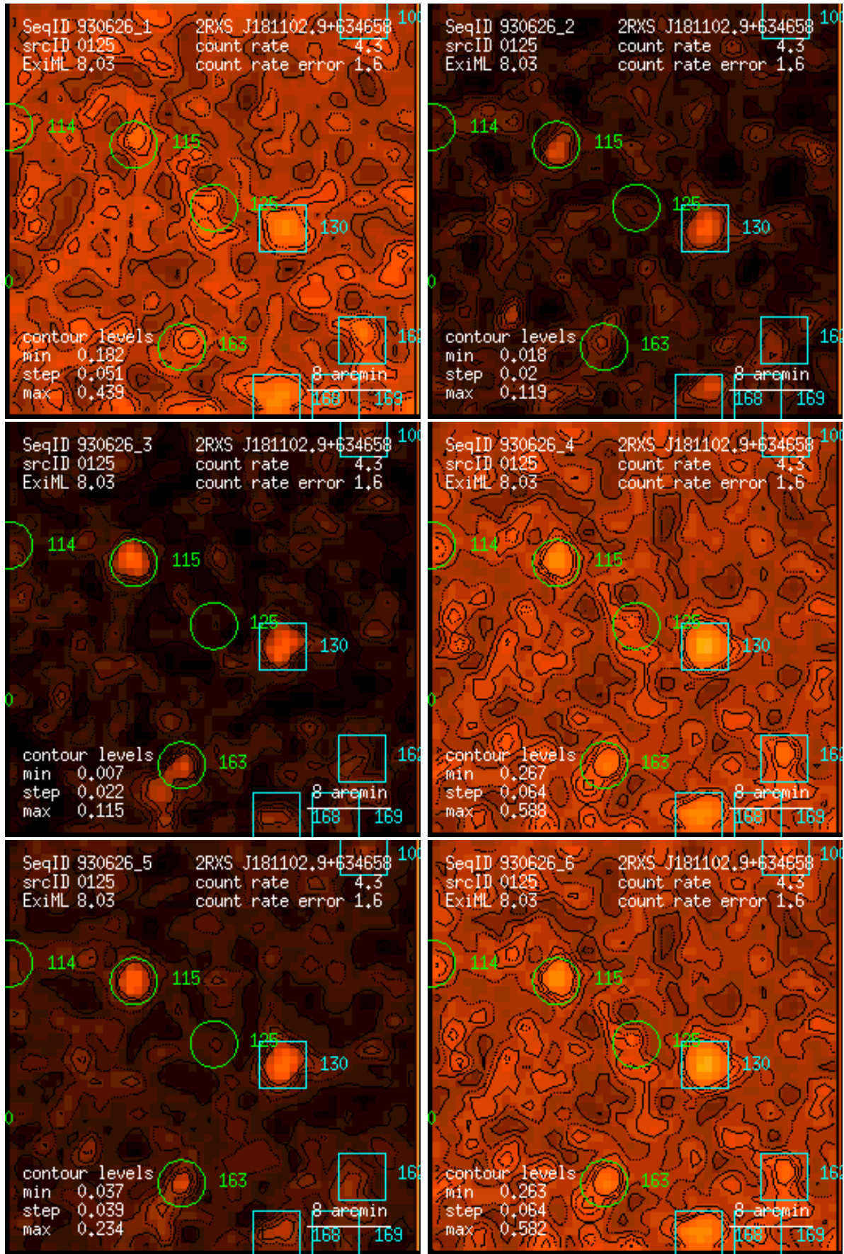
Figure 125: RASS 930626: detection 0125: band rate images, Gaussian filter: (1) PSPC channels 11 – 41, (2) 52 – 90, (3) 91 – 201, (4) 11 – 235, (5) 52 – 201, (6) 11 – 201. Broad band rates in counts/ks. Band rate contour levels in counts/ks/arcmin 2 .
