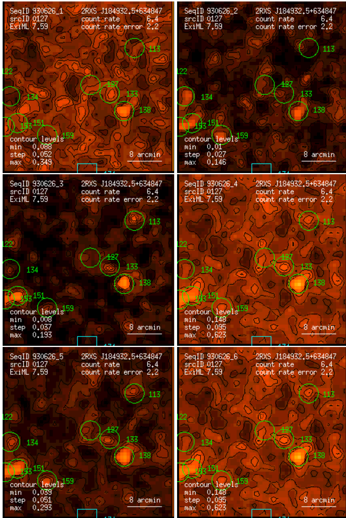
Figure 127: RASS 930626: detection 0127: band rate images, Gaussian filter: (1) PSPC channels 11 – 41, (2) 52 – 90, (3) 91 – 201, (4) 11 – 235, (5) 52 – 201, (6) 11 – 201. Broad band rates in counts/ks. Band rate contour levels in counts/ks/arcmin 2 .
