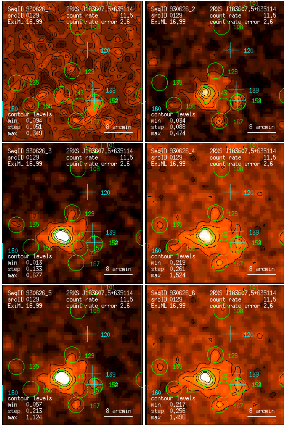
Figure 129: RASS 930626: detection 0129: band rate images, Gaussian filter: (1) PSPC channels 11 – 41, (2) 52 – 90, (3) 91 – 201, (4) 11 – 235, (5) 52 – 201, (6) 11 – 201. Broad band rates in counts/ks. Band rate contour levels in counts/ks/arcmin 2 .
