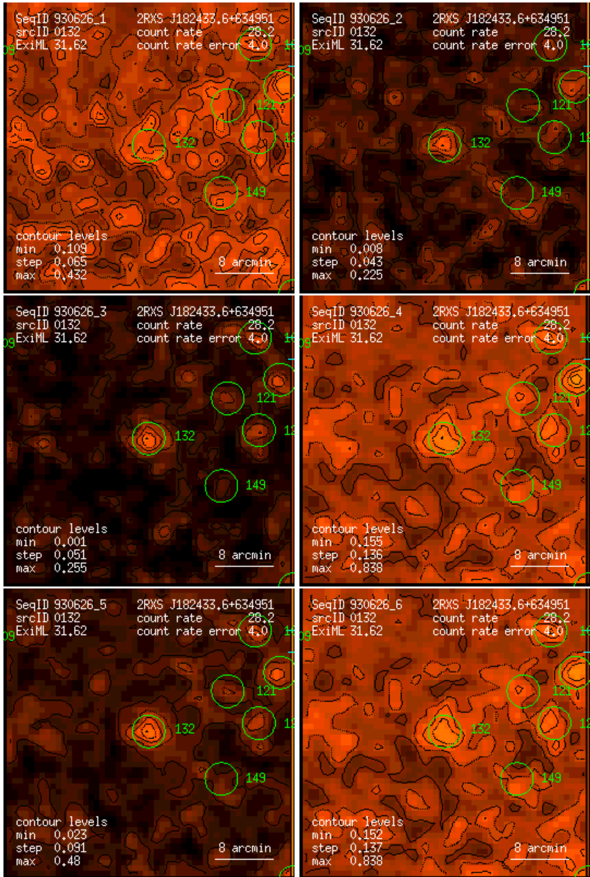
Figure 132: RASS 930626: detection 0132: band rate images, Gaussian filter: (1) PSPC channels 11 – 41, (2) 52 – 90, (3) 91 – 201, (4) 11 – 235, (5) 52 – 201, (6) 11 – 201. Broad band rates in counts/ks. Band rate contour levels in counts/ks/arcmin 2 .
