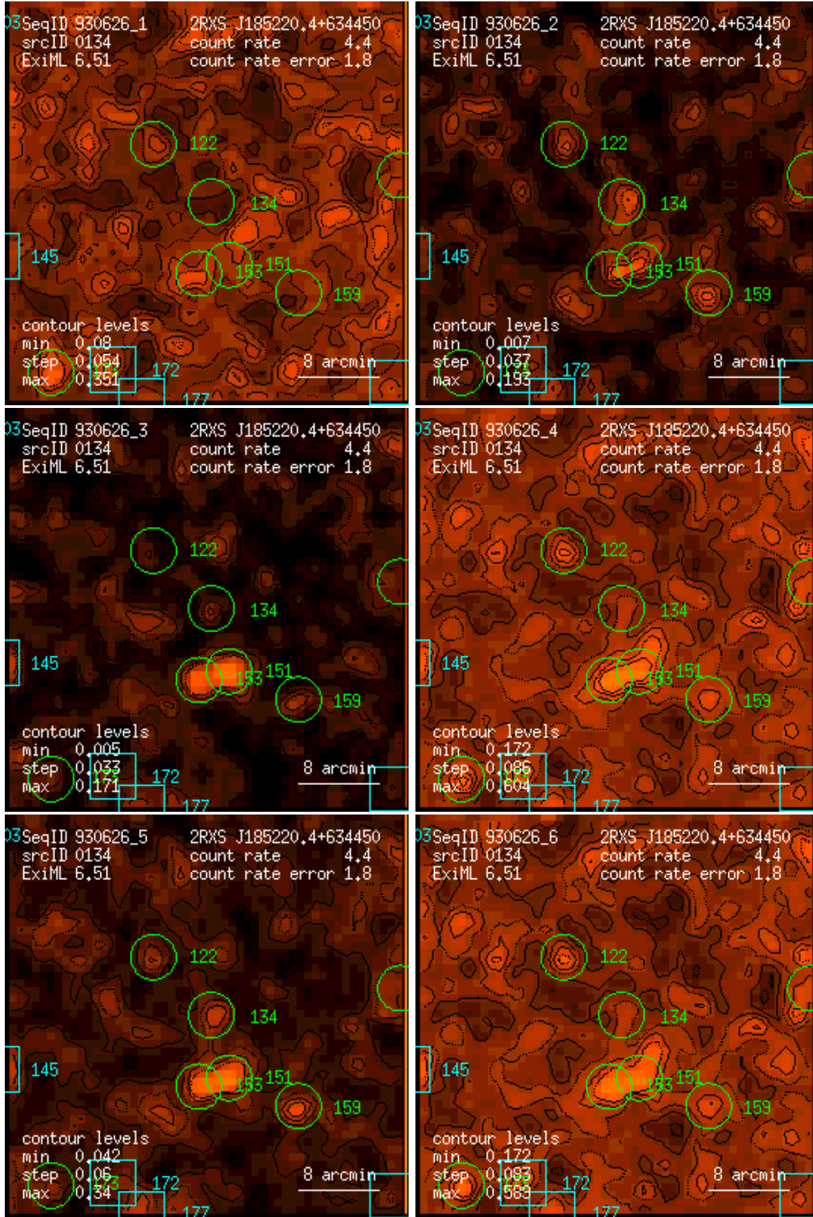
Figure 134: RASS 930626: detection 0134: band rate images, Gaussian filter: (1) PSPC channels 11 – 41, (2) 52 – 90, (3) 91 – 201, (4) 11 – 235, (5) 52 – 201, (6) 11 – 201. Broad band rates in counts/ks. Band rate contour levels in counts/ks/arcmin 2 .
