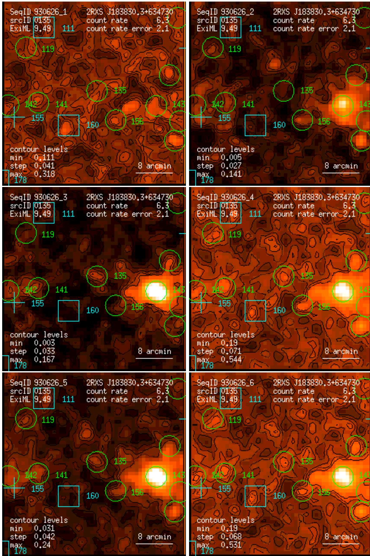
Figure 135: RASS 930626: detection 0135: band rate images, Gaussian filter: (1) PSPC channels 11 – 41, (2) 52 – 90, (3) 91 – 201, (4) 11 – 235, (5) 52 – 201, (6) 11 – 201. Broad band rates in counts/ks. Band rate contour levels in counts/ks/arcmin 2 .
