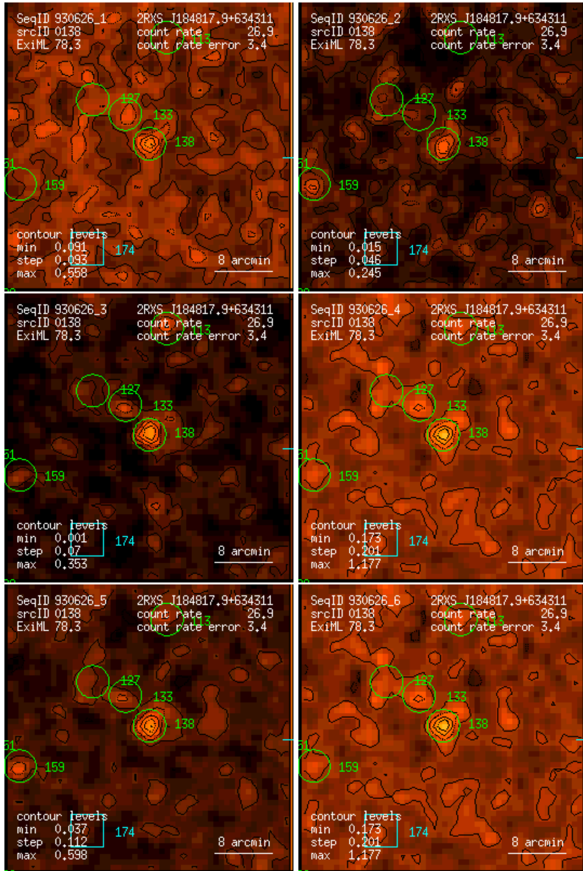
Figure 138: RASS 930626: detection 0138: band rate images, Gaussian filter: (1) PSPC channels 11 – 41, (2) 52 – 90, (3) 91 – 201, (4) 11 – 235, (5) 52 – 201, (6) 11 – 201. Broad band rates in counts/ks. Band rate contour levels in counts/ks/arcmin 2 .
