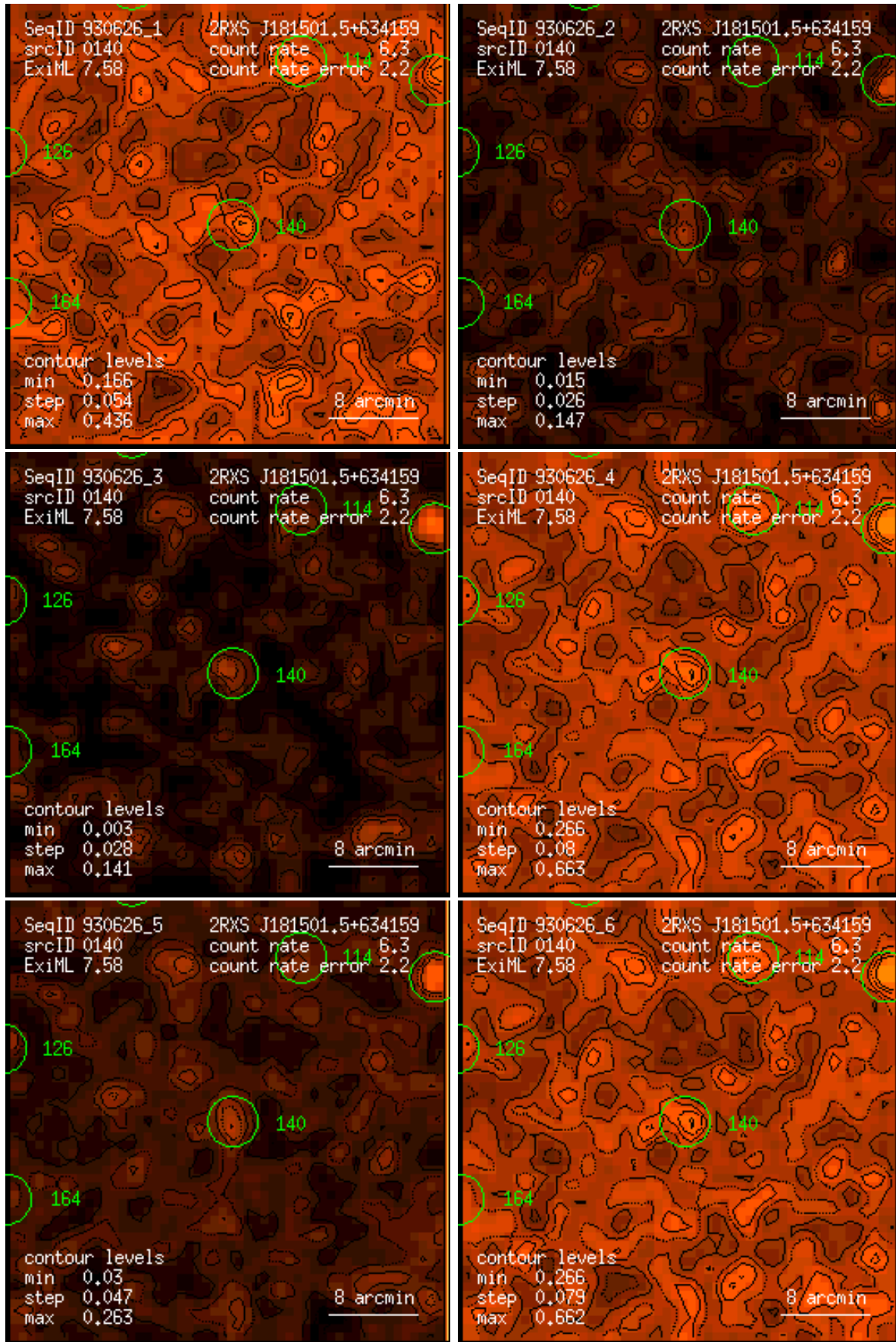
Figure 140: RASS 930626: detection 0140: band rate images, Gaussian filter: (1) PSPC channels 11 – 41, (2) 52 – 90, (3) 91 – 201, (4) 11 – 235, (5) 52 – 201, (6) 11 – 201. Broad band rates in counts/ks. Band rate contour levels in counts/ks/arcmin 2 .
