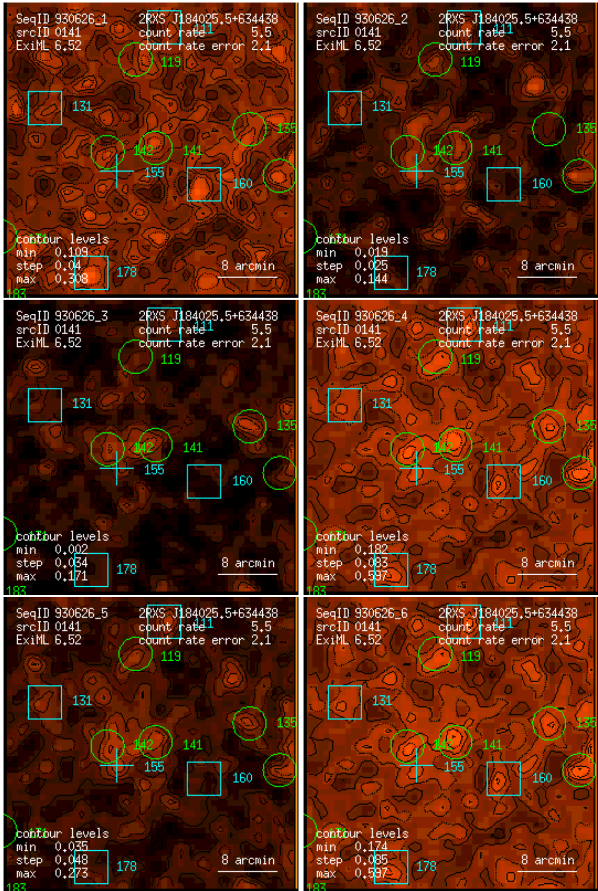
Figure 141: RASS 930626: detection 0141: band rate images, Gaussian filter: (1) PSPC channels 11 – 41, (2) 52 – 90, (3) 91 – 201, (4) 11 – 235, (5) 52 – 201, (6) 11 – 201. Broad band rates in counts/ks. Band rate contour levels in counts/ks/arcmin 2 .
