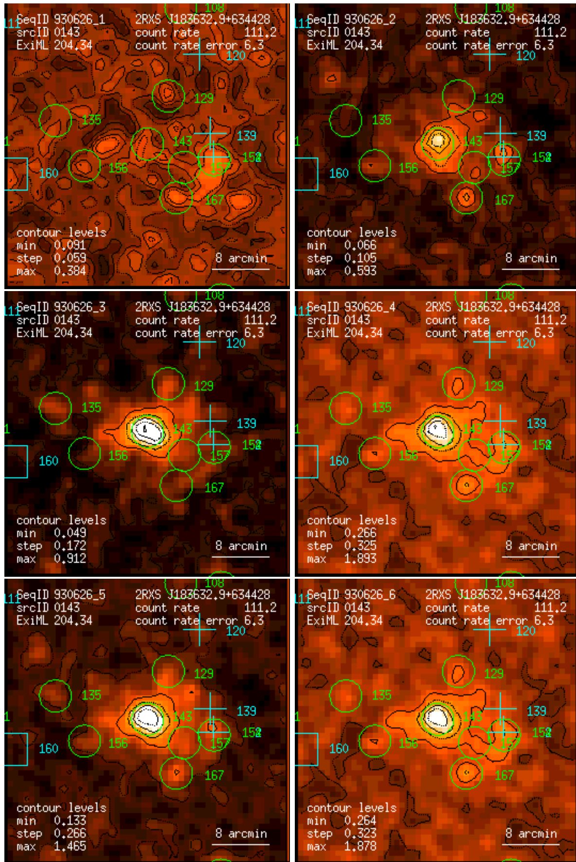
Figure 143: RASS 930626: detection 0143: band rate images, Gaussian filter: (1) PSPC channels 11 – 41, (2) 52 – 90, (3) 91 – 201, (4) 11 – 235, (5) 52 – 201, (6) 11 – 201. Broad band rates in counts/ks. Band rate contour levels in counts/ks/arcmin 2 .
