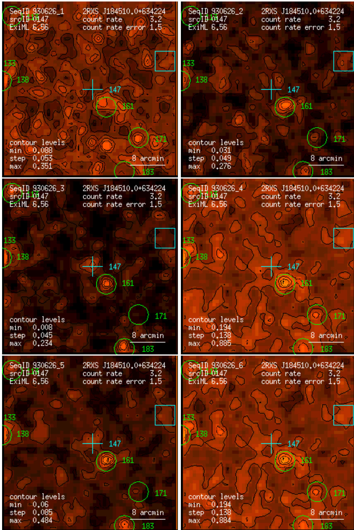
Figure 147: RASS 930626: detection 0147: band rate images, Gaussian filter: (1) PSPC channels 11 – 41, (2) 52 – 90, (3) 91 – 201, (4) 11 – 235, (5) 52 – 201, (6) 11 – 201. Broad band rates in counts/ks. Band rate contour levels in counts/ks/arcmin 2 .
