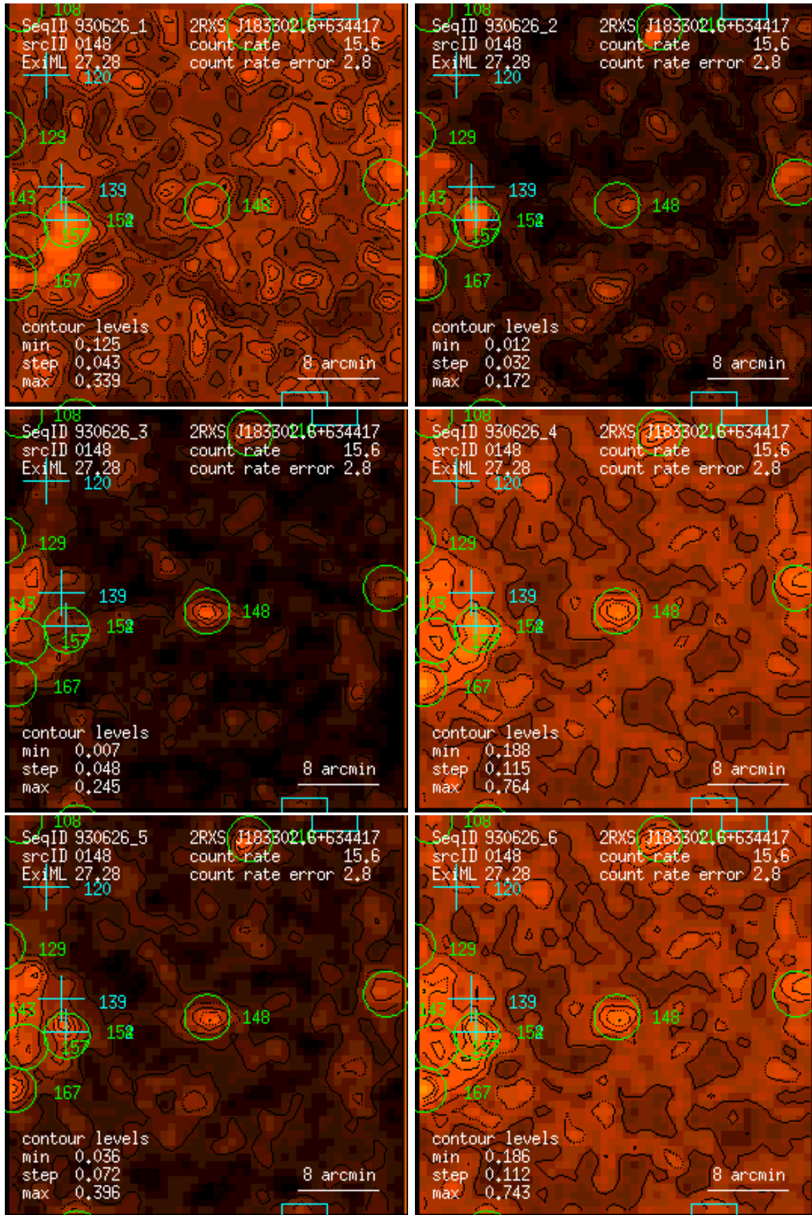
Figure 148: RASS 930626: detection 0148: band rate images, Gaussian filter: (1) PSPC channels 11 – 41, (2) 52 – 90, (3) 91 – 201, (4) 11 – 235, (5) 52 – 201, (6) 11 – 201. Broad band rates in counts/ks. Band rate contour levels in counts/ks/arcmin 2 .
