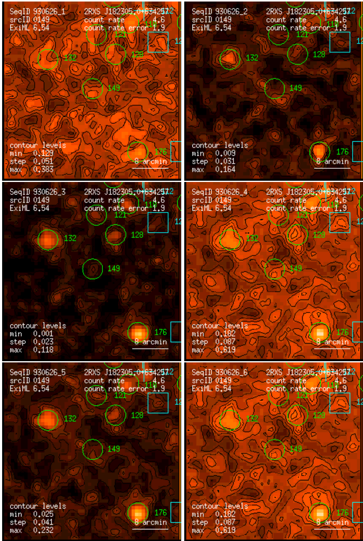
Figure 149: RASS 930626: detection 0149: band rate images, Gaussian filter: (1) PSPC channels 11 – 41, (2) 52 – 90, (3) 91 – 201, (4) 11 – 235, (5) 52 – 201, (6) 11 – 201. Broad band rates in counts/ks. Band rate contour levels in counts/ks/arcmin 2 .
