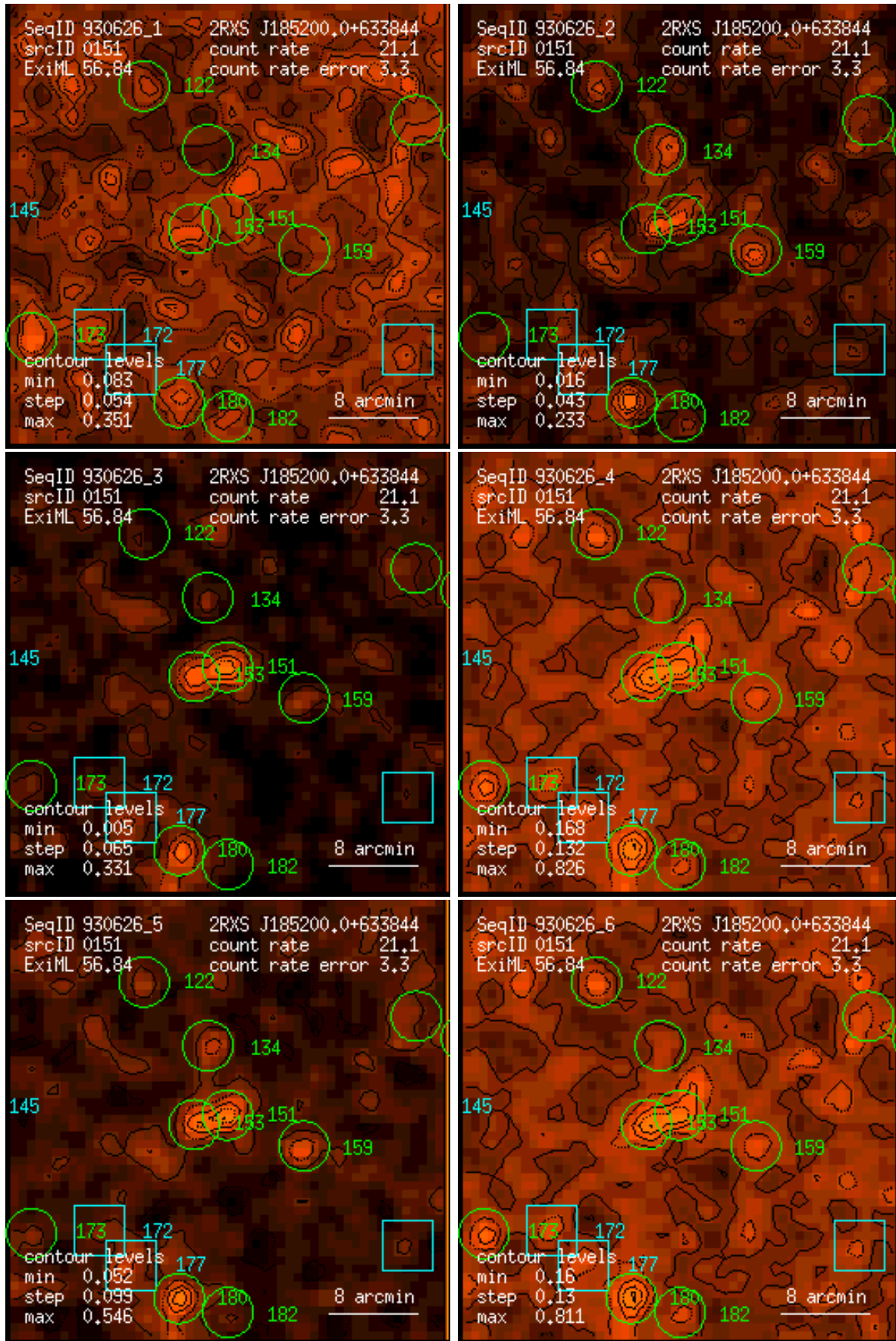
Figure 151: RASS 930626: detection 0151: band rate images, Gaussian filter: (1) PSPC channels 11 – 41, (2) 52 – 90, (3) 91 – 201, (4) 11 – 235, (5) 52 – 201, (6) 11 – 201. Broad band rates in counts/ks. Band rate contour levels in counts/ks/arcmin 2 .
