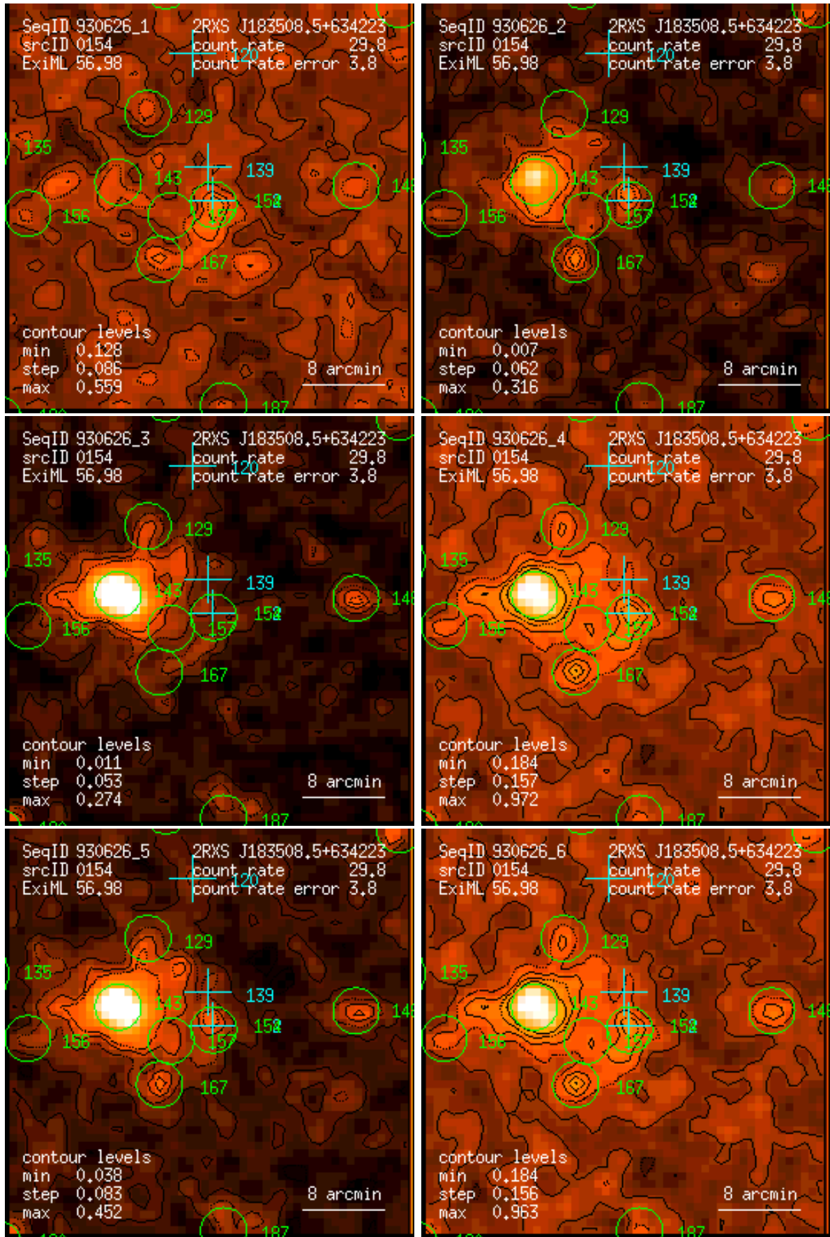
Figure 154: RASS 930626: detection 0154: band rate images, Gaussian filter: (1) PSPC channels 11 – 41, (2) 52 – 90, (3) 91 – 201, (4) 11 – 235, (5) 52 – 201, (6) 11 – 201. Broad band rates in counts/ks. Band rate contour levels in counts/ks/arcmin 2 .
