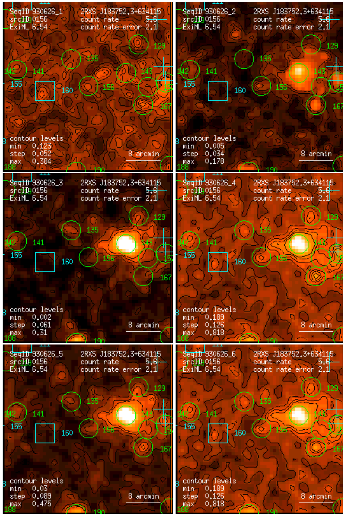
Figure 156: RASS 930626: detection 0156: band rate images, Gaussian filter: (1) PSPC channels 11 – 41, (2) 52 – 90, (3) 91 – 201, (4) 11 – 235, (5) 52 – 201, (6) 11 – 201. Broad band rates in counts/ks. Band rate contour levels in counts/ks/arcmin 2 .
