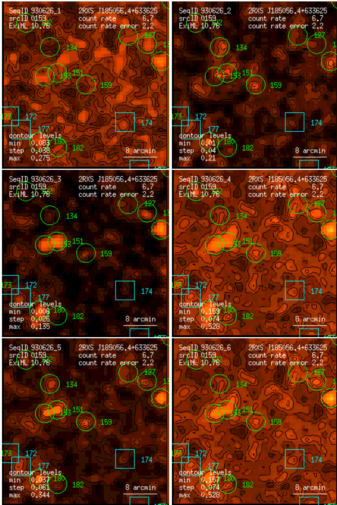
Figure 159: RASS 930626: detection 0159: band rate images, Gaussian filter: (1) PSPC channels 11 – 41, (2) 52 – 90, (3) 91 – 201, (4) 11 – 235, (5) 52 – 201, (6) 11 – 201. Broad band rates in counts/ks. Band rate contour levels in counts/ks/arcmin 2 .
