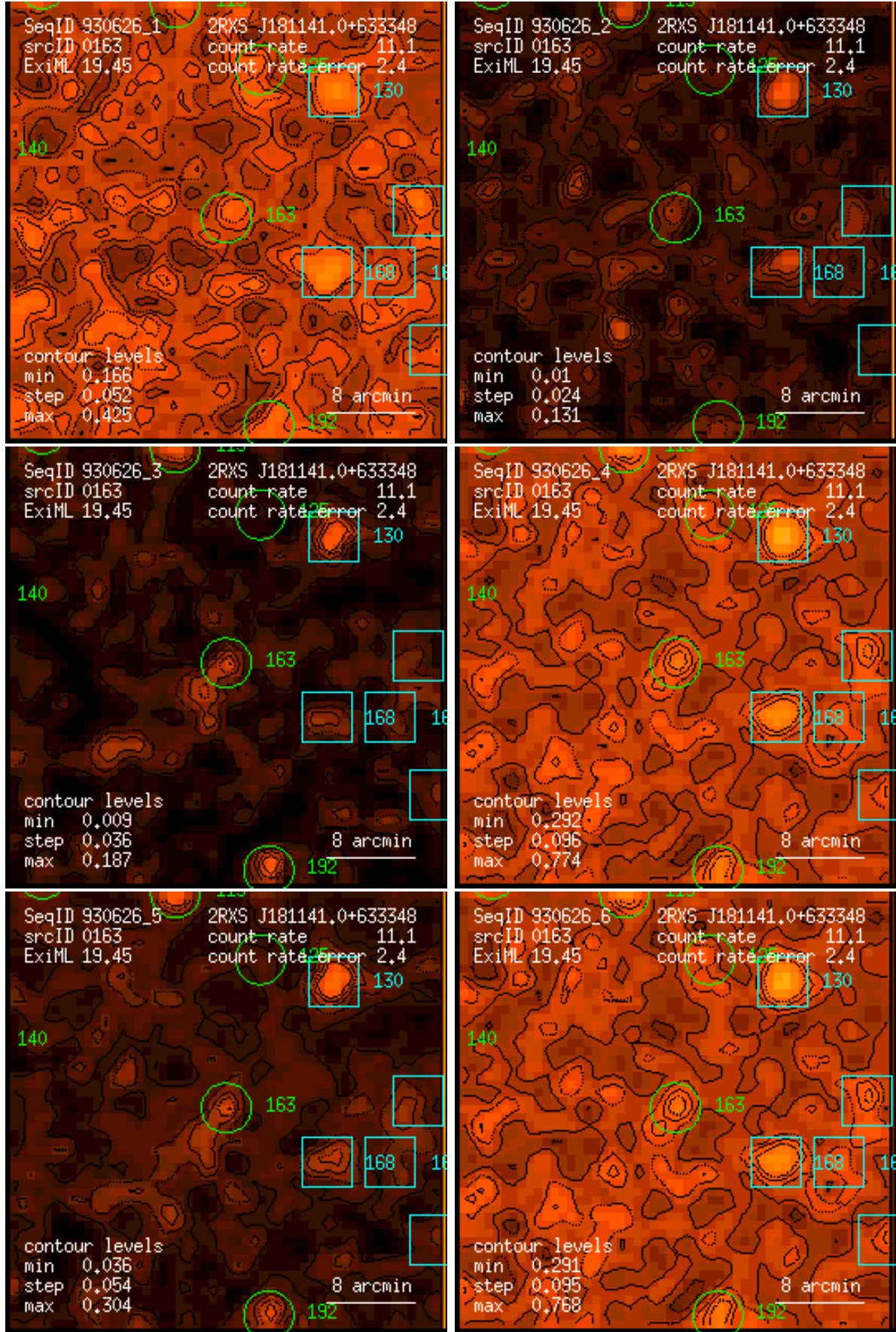
Figure 163: RASS 930626: detection 0163: band rate images, Gaussian filter: (1) PSPC channels 11 – 41, (2) 52 – 90, (3) 91 – 201, (4) 11 – 235, (5) 52 – 201, (6) 11 – 201. Broad band rates in counts/ks. Band rate contour levels in counts/ks/arcmin 2 .
