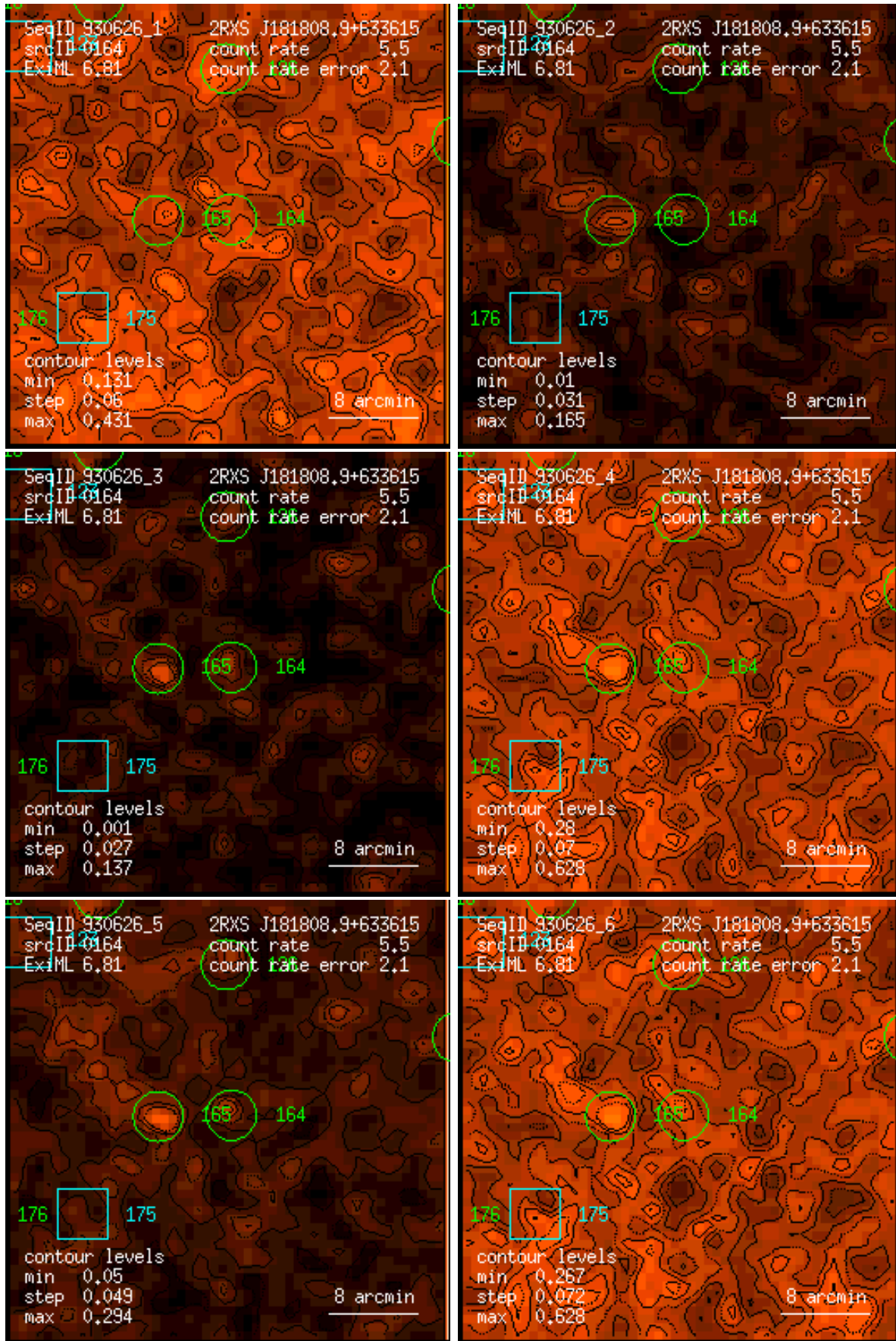
Figure 164: RASS 930626: detection 0164: band rate images, Gaussian filter: (1) PSPC channels 11 – 41, (2) 52 – 90, (3) 91 – 201, (4) 11 – 235, (5) 52 – 201, (6) 11 – 201. Broad band rates in counts/ks. Band rate contour levels in counts/ks/arcmin 2 .
