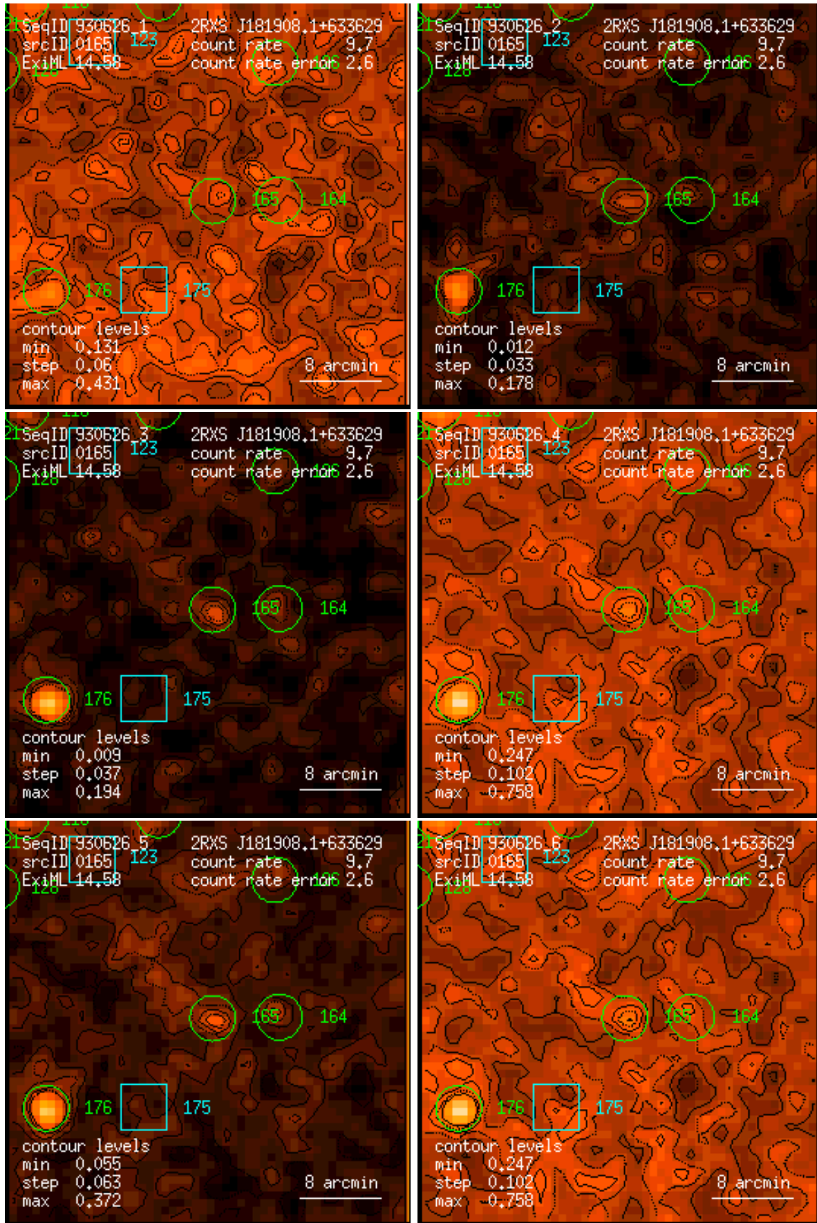
Figure 165: RASS 930626: detection 0165: band rate images, Gaussian filter: (1) PSPC channels 11 – 41, (2) 52 – 90, (3) 91 – 201, (4) 11 – 235, (5) 52 – 201, (6) 11 – 201. Broad band rates in counts/ks. Band rate contour levels in counts/ks/arcmin 2 .
