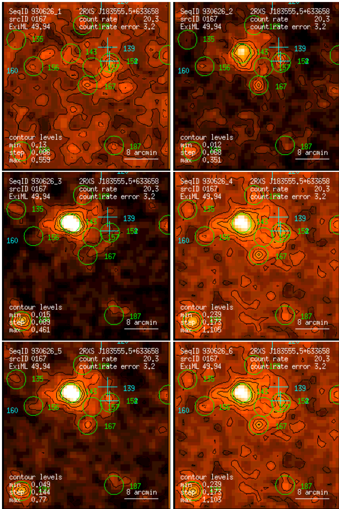
Figure 167: RASS 930626: detection 0167: band rate images, Gaussian filter: (1) PSPC channels 11 – 41, (2) 52 – 90, (3) 91 – 201, (4) 11 – 235, (5) 52 – 201, (6) 11 – 201. Broad band rates in counts/ks. Band rate contour levels in counts/ks/arcmin 2 .
