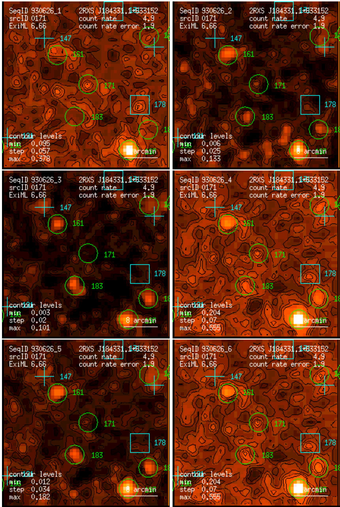
Figure 171: RASS 930626: detection 0171: band rate images, Gaussian filter: (1) PSPC channels 11 – 41, (2) 52 – 90, (3) 91 – 201, (4) 11 – 235, (5) 52 – 201, (6) 11 – 201. Broad band rates in counts/ks. Band rate contour levels in counts/ks/arcmin 2 .
