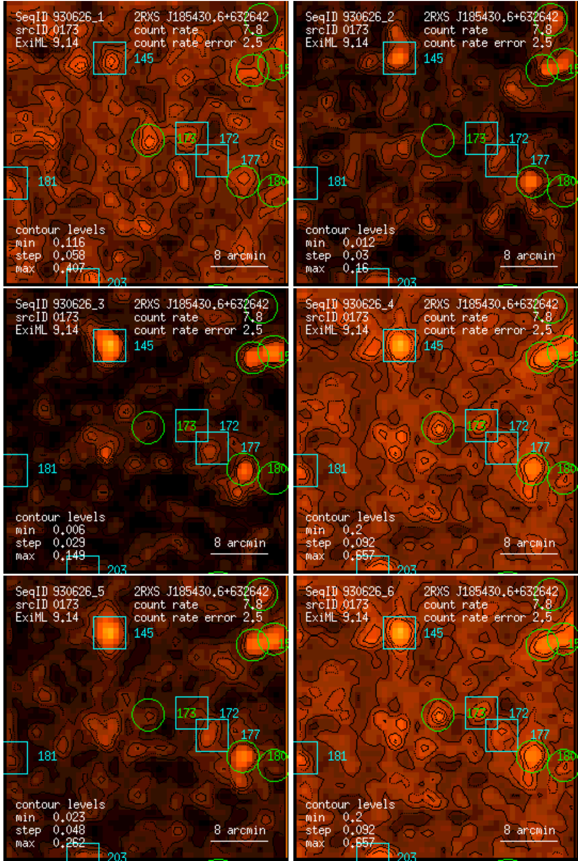
Figure 173: RASS 930626: detection 0173: band rate images, Gaussian filter: (1) PSPC channels 11 – 41, (2) 52 – 90, (3) 91 – 201, (4) 11 – 235, (5) 52 – 201, (6) 11 – 201. Broad band rates in counts/ks. Band rate contour levels in counts/ks/arcmin 2 .
