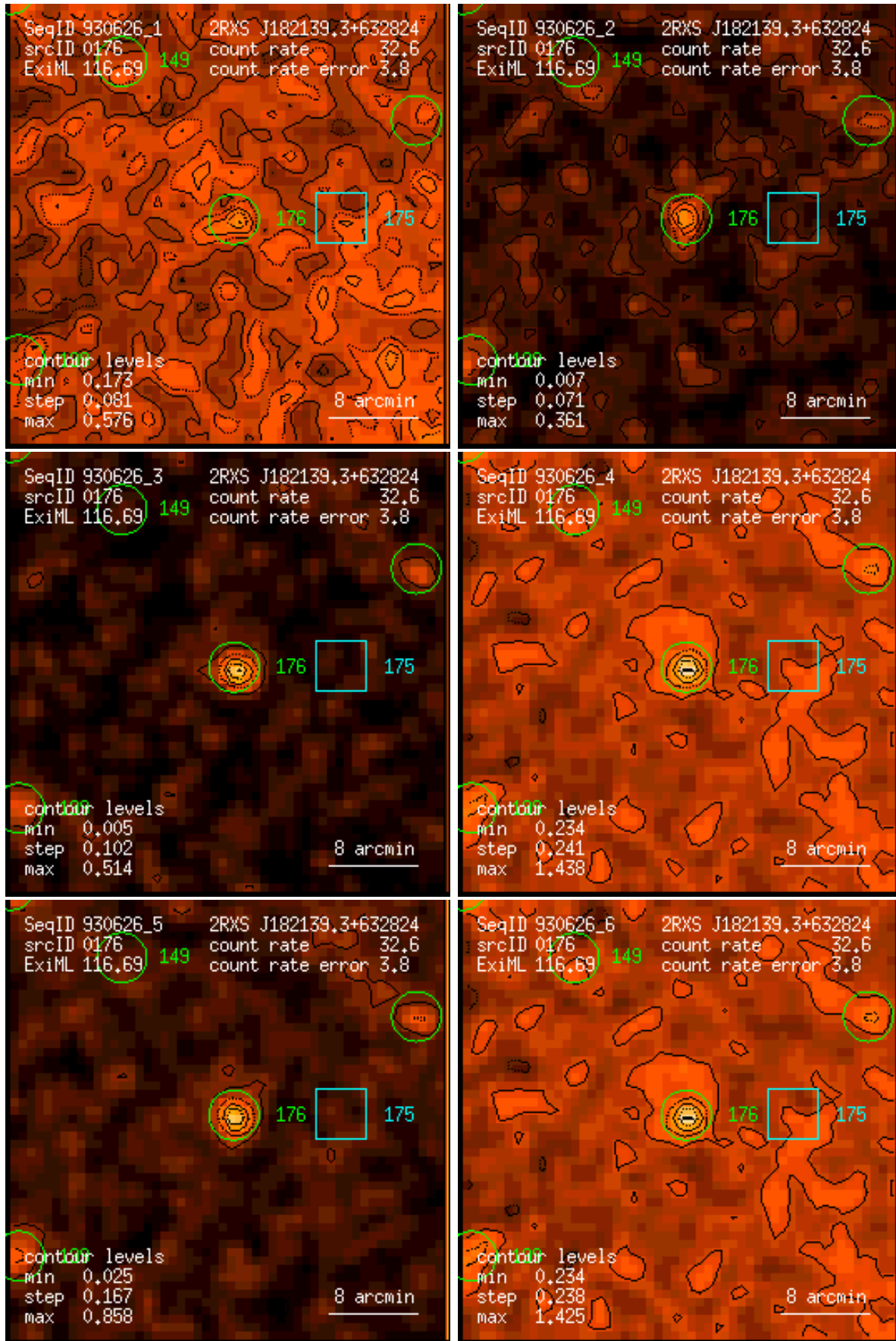
Figure 176: RASS 930626: detection 0176: band rate images, Gaussian filter: (1) PSPC channels 11 – 41, (2) 52 – 90, (3) 91 – 201, (4) 11 – 235, (5) 52 – 201, (6) 11 – 201. Broad band rates in counts/ks. Band rate contour levels in counts/ks/arcmin 2 .
