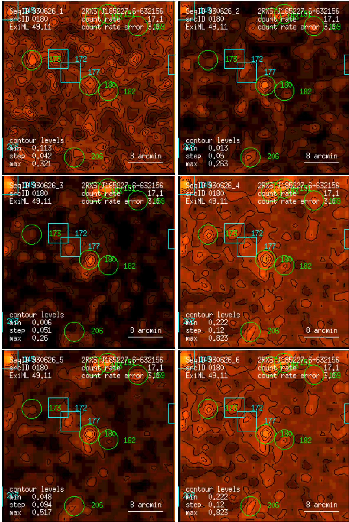
Figure 180: RASS 930626: detection 0180: band rate images, Gaussian filter: (1) PSPC channels 11 – 41, (2) 52 – 90, (3) 91 – 201, (4) 11 – 235, (5) 52 – 201, (6) 11 – 201. Broad band rates in counts/ks. Band rate contour levels in counts/ks/arcmin 2 .
