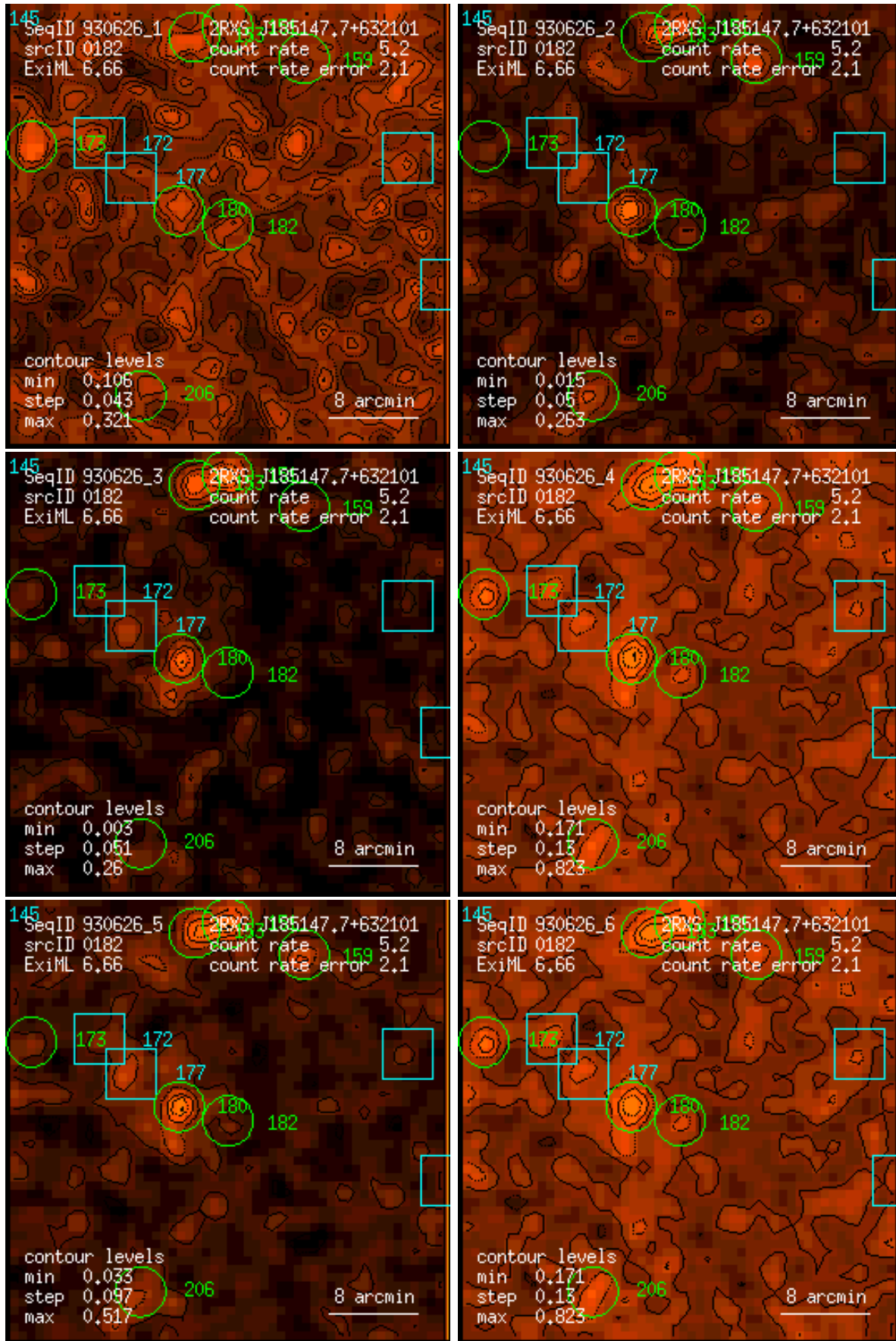
Figure 182: RASS 930626: detection 0182: band rate images, Gaussian filter: (1) PSPC channels 11 – 41, (2) 52 – 90, (3) 91 – 201, (4) 11 – 235, (5) 52 – 201, (6) 11 – 201. Broad band rates in counts/ks. Band rate contour levels in counts/ks/arcmin 2 .
