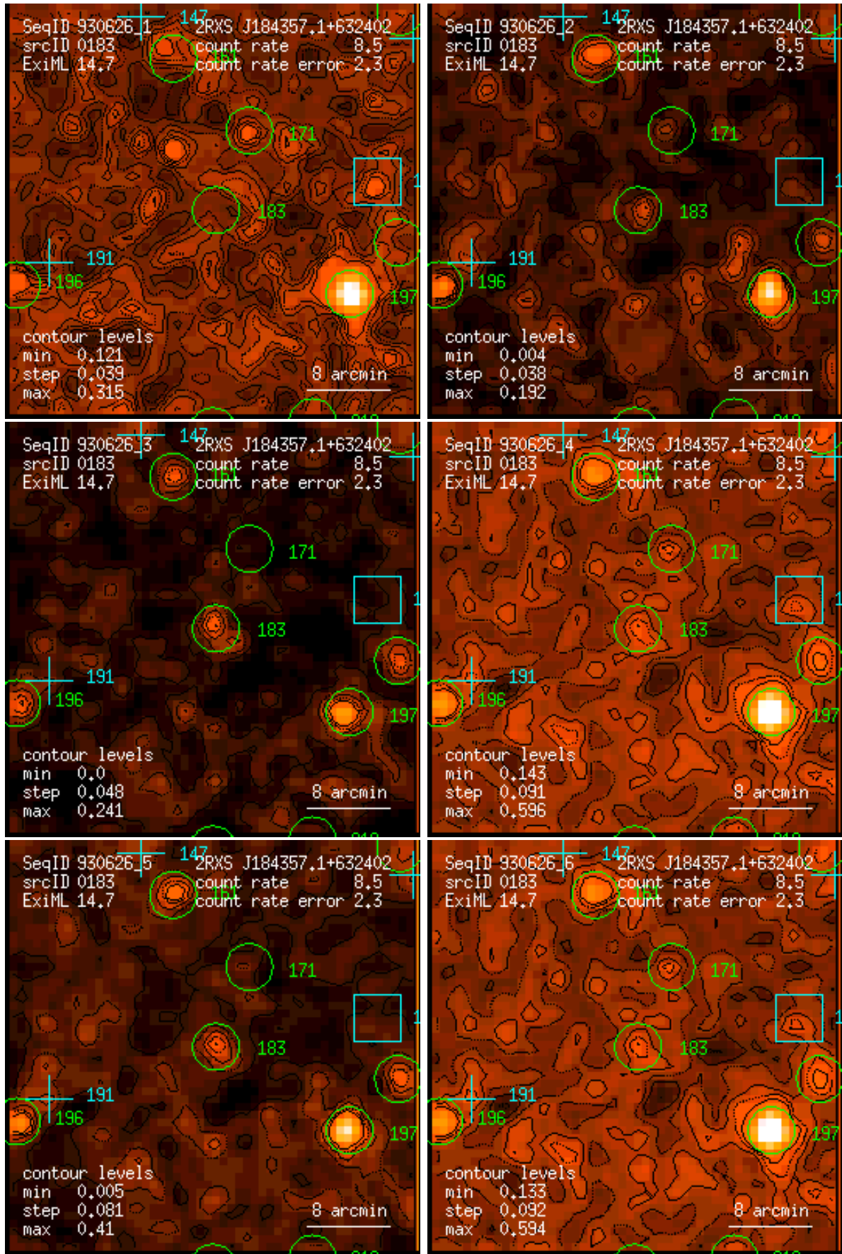
Figure 183: RASS 930626: detection 0183: band rate images, Gaussian filter: (1) PSPC channels 11 – 41, (2) 52 – 90, (3) 91 – 201, (4) 11 – 235, (5) 52 – 201, (6) 11 – 201. Broad band rates in counts/ks. Band rate contour levels in counts/ks/arcmin 2 .
