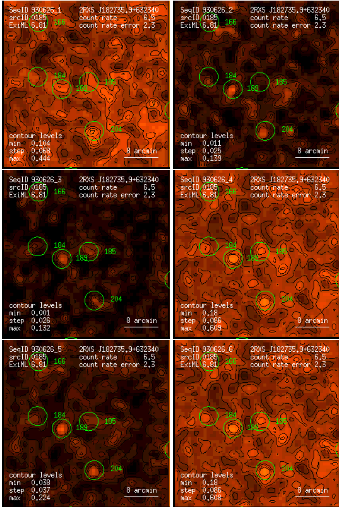
Figure 185: RASS 930626: detection 0185: band rate images, Gaussian filter: (1) PSPC channels 11 – 41, (2) 52 – 90, (3) 91 – 201, (4) 11 – 235, (5) 52 – 201, (6) 11 – 201. Broad band rates in counts/ks. Band rate contour levels in counts/ks/arcmin 2 .
