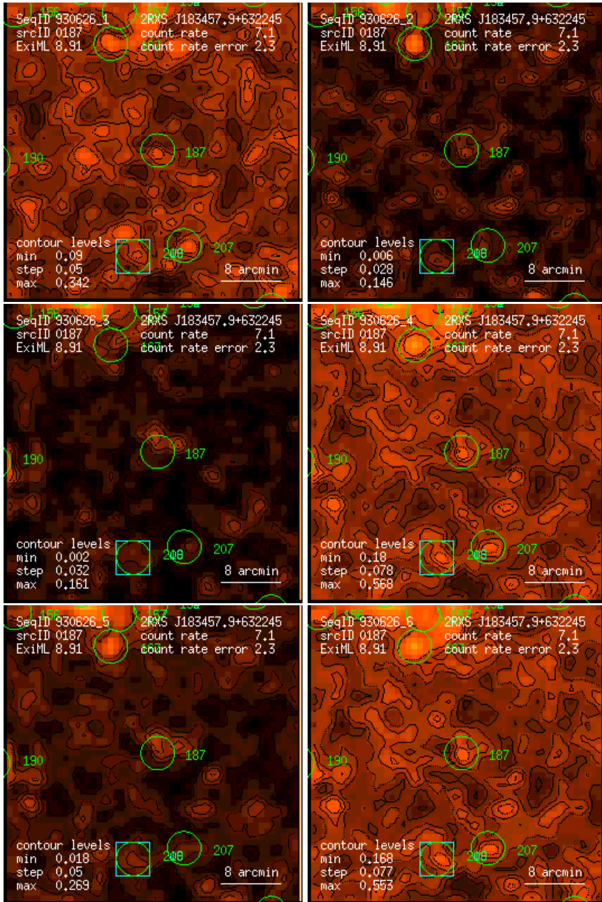
Figure 187: RASS 930626: detection 0187: band rate images, Gaussian filter: (1) PSPC channels 11 – 41, (2) 52 – 90, (3) 91 – 201, (4) 11 – 235, (5) 52 – 201, (6) 11 – 201. Broad band rates in counts/ks. Band rate contour levels in counts/ks/arcmin 2 .
