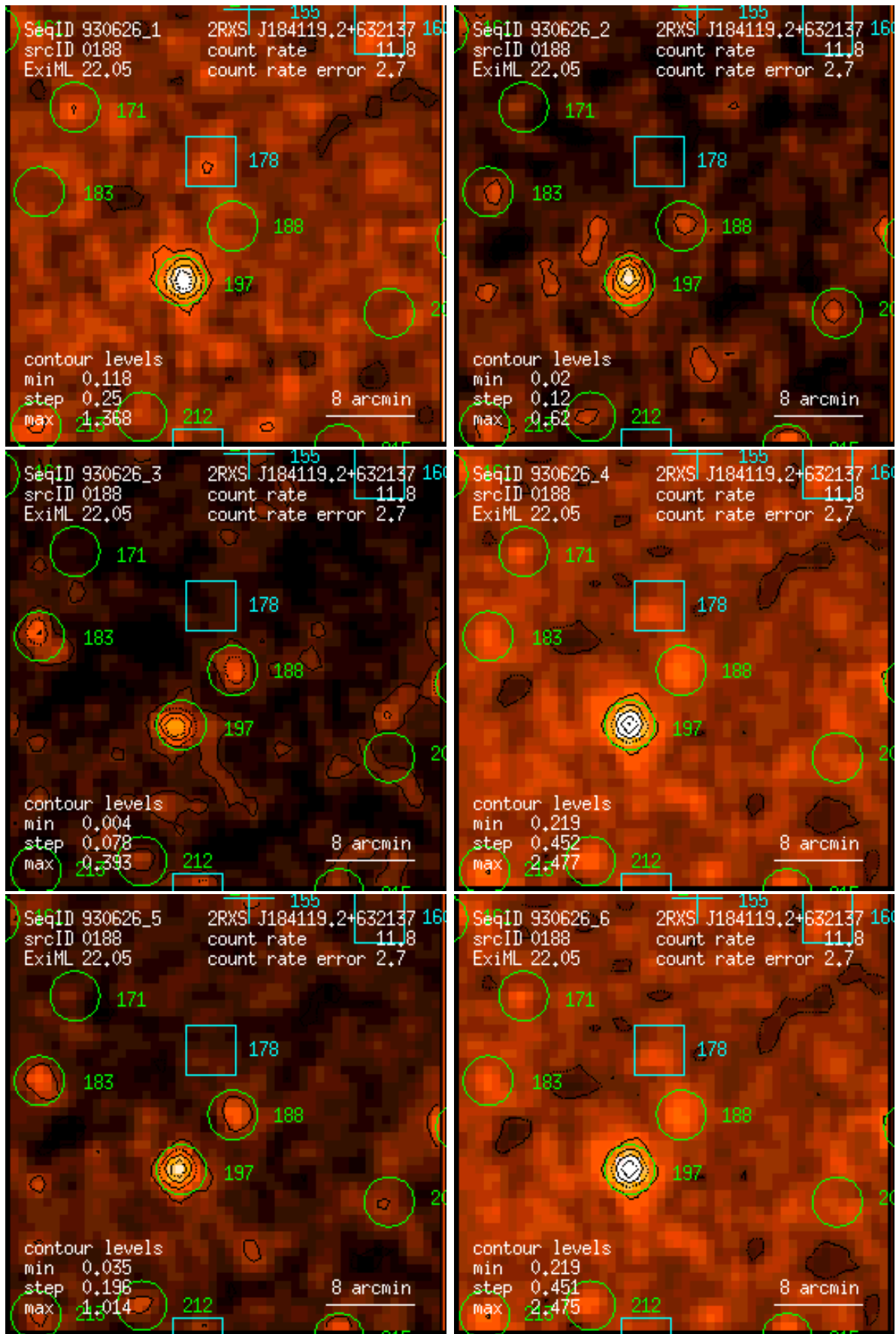
Figure 188: RASS 930626: detection 0188: band rate images, Gaussian filter: (1) PSPC channels 11 – 41, (2) 52 – 90, (3) 91 – 201, (4) 11 – 235, (5) 52 – 201, (6) 11 – 201. Broad band rates in counts/ks. Band rate contour levels in counts/ks/arcmin 2 .
