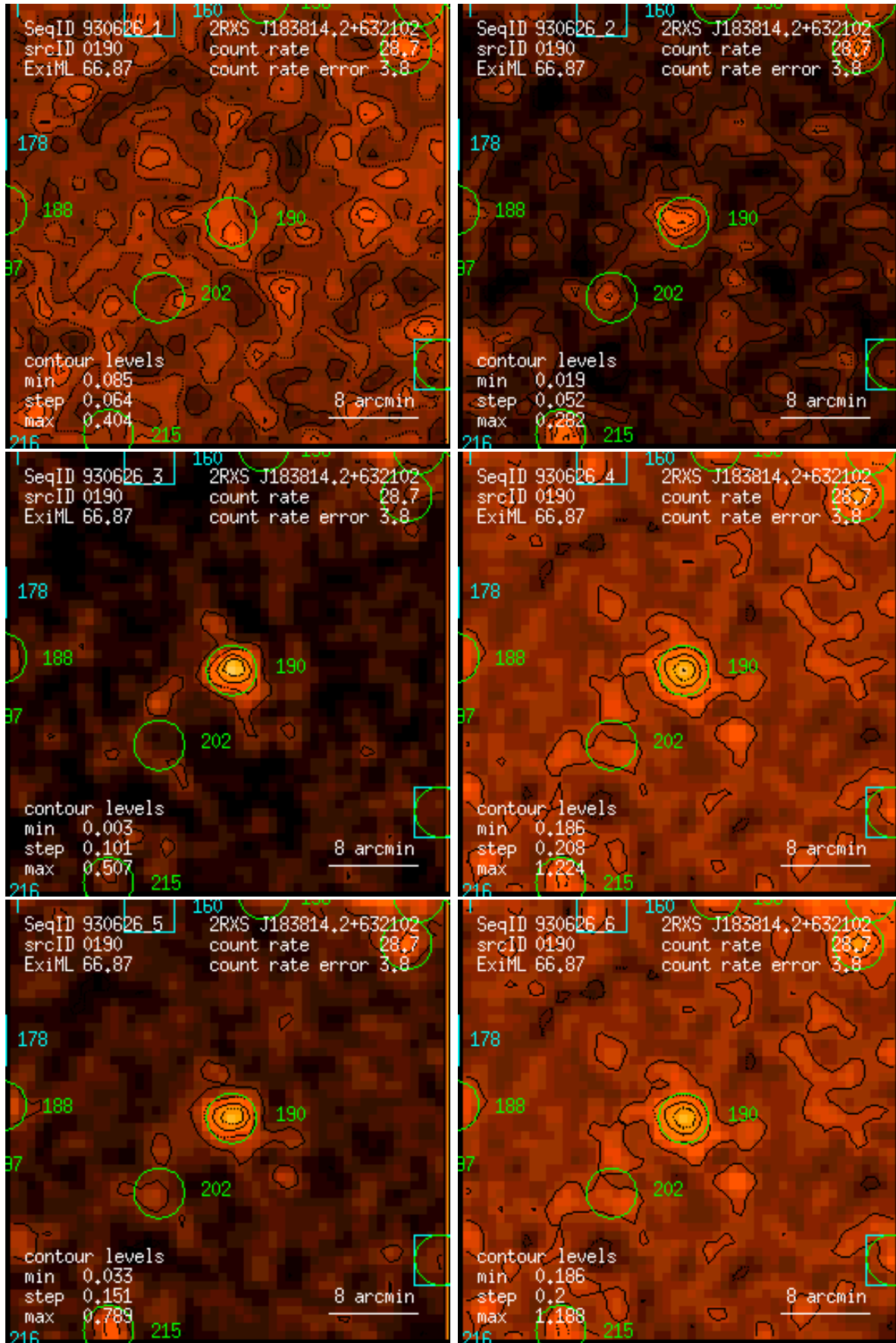
Figure 190: RASS 930626: detection 0190: band rate images, Gaussian filter: (1) PSPC channels 11 – 41, (2) 52 – 90, (3) 91 – 201, (4) 11 – 235, (5) 52 – 201, (6) 11 – 201. Broad band rates in counts/ks. Band rate contour levels in counts/ks/arcmin 2 .
