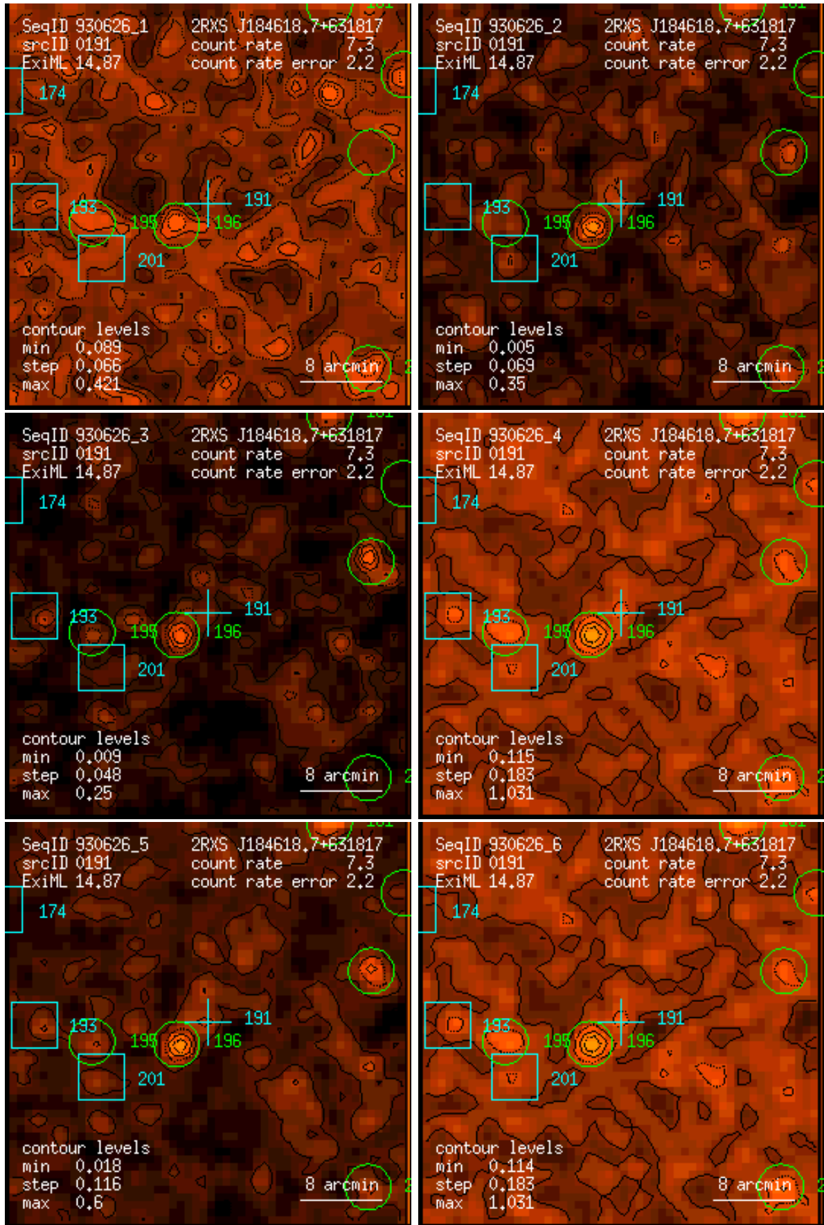
Figure 191: RASS 930626: detection 0191: band rate images, Gaussian filter: (1) PSPC channels 11 – 41, (2) 52 – 90, (3) 91 – 201, (4) 11 – 235, (5) 52 – 201, (6) 11 – 201. Broad band rates in counts/ks. Band rate contour levels in counts/ks/arcmin 2 .
