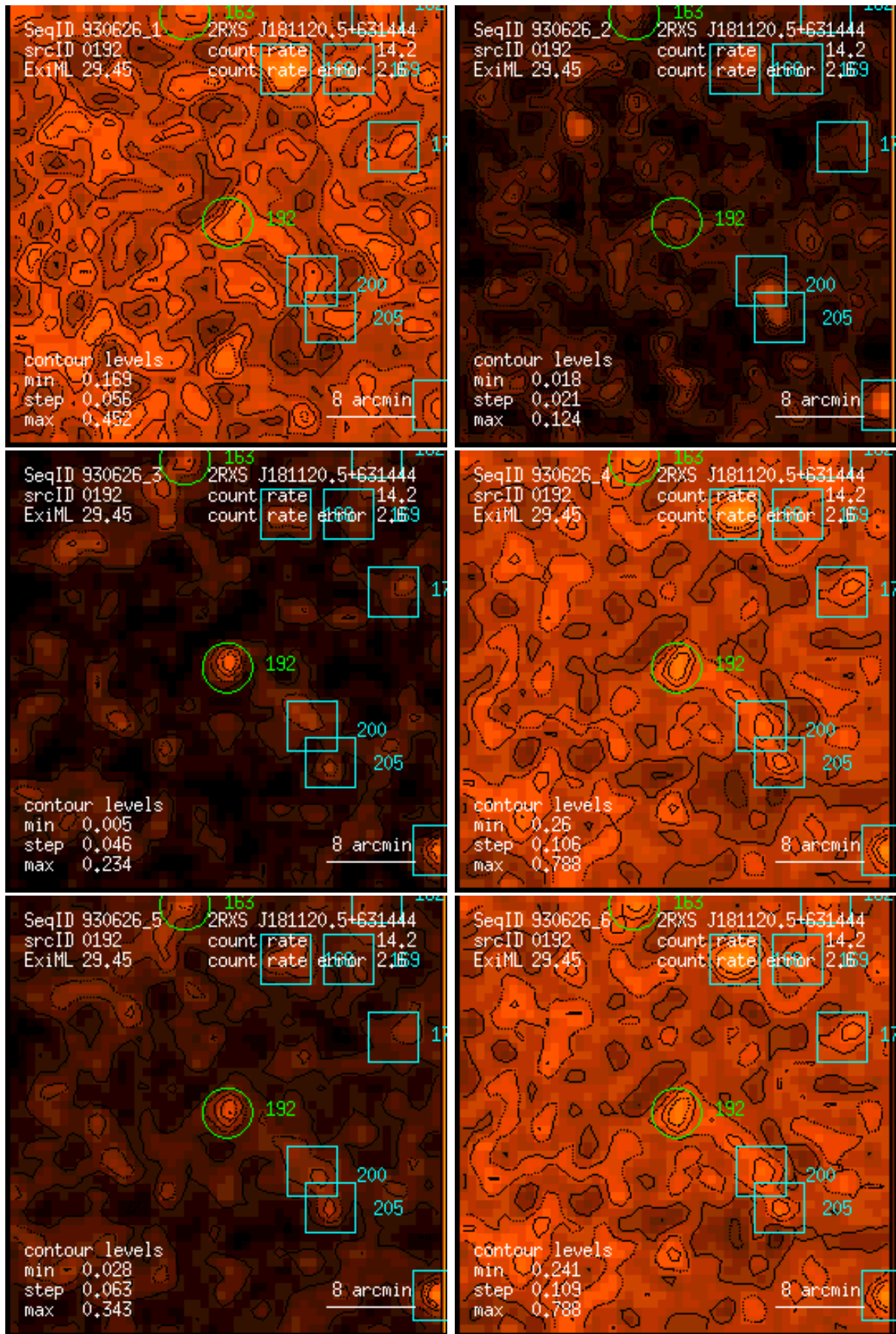
Figure 192: RASS 930626: detection 0192: band rate images, Gaussian filter: (1) PSPC channels 11 – 41, (2) 52 – 90, (3) 91 – 201, (4) 11 – 235, (5) 52 – 201, (6) 11 – 201. Broad band rates in counts/ks. Band rate contour levels in counts/ks/arcmin 2 .
