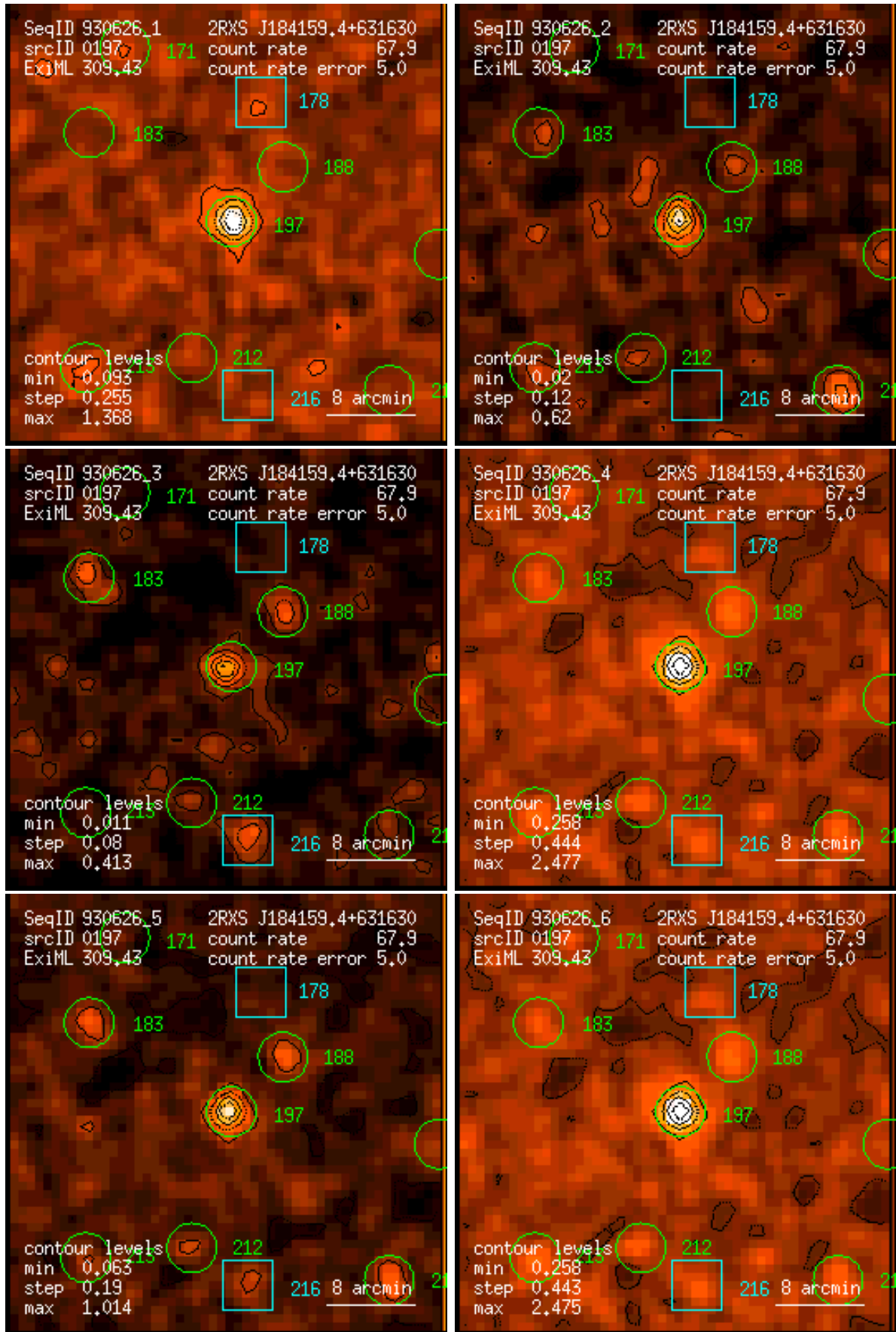
Figure 197: RASS 930626: detection 0197: band rate images, Gaussian filter: (1) PSPC channels 11 – 41, (2) 52 – 90, (3) 91 – 201, (4) 11 – 235, (5) 52 – 201, (6) 11 – 201. Broad band rates in counts/ks. Band rate contour levels in counts/ks/arcmin 2 .
