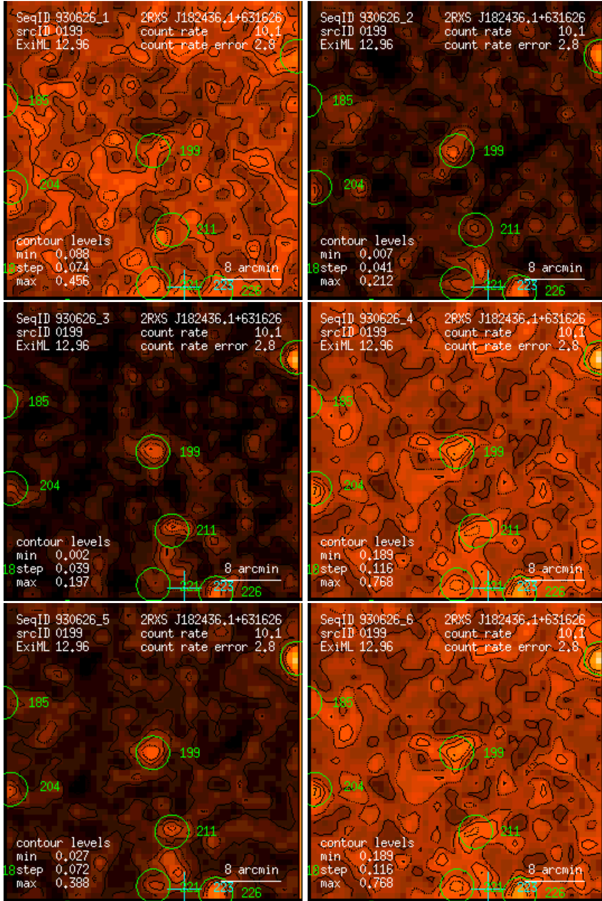
Figure 199: RASS 930626: detection 0199: band rate images, Gaussian filter: (1) PSPC channels 11 – 41, (2) 52 – 90, (3) 91 – 201, (4) 11 – 235, (5) 52 – 201, (6) 11 – 201. Broad band rates in counts/ks. Band rate contour levels in counts/ks/arcmin 2 .
