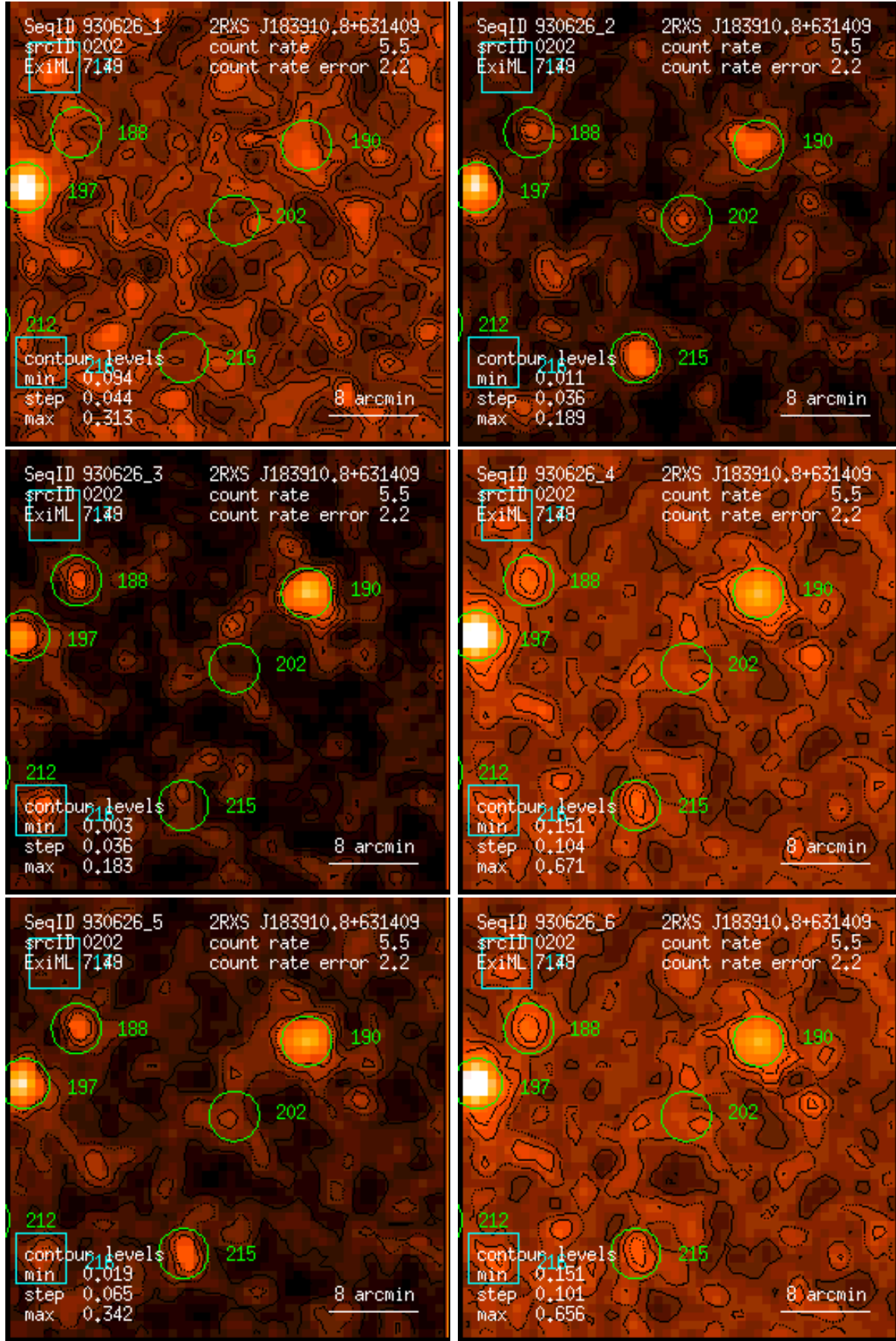
Figure 202: RASS 930626: detection 0202: band rate images, Gaussian filter: (1) PSPC channels 11 – 41, (2) 52 – 90, (3) 91 – 201, (4) 11 – 235, (5) 52 – 201, (6) 11 – 201. Broad band rates in counts/ks. Band rate contour levels in counts/ks/arcmin 2 .
