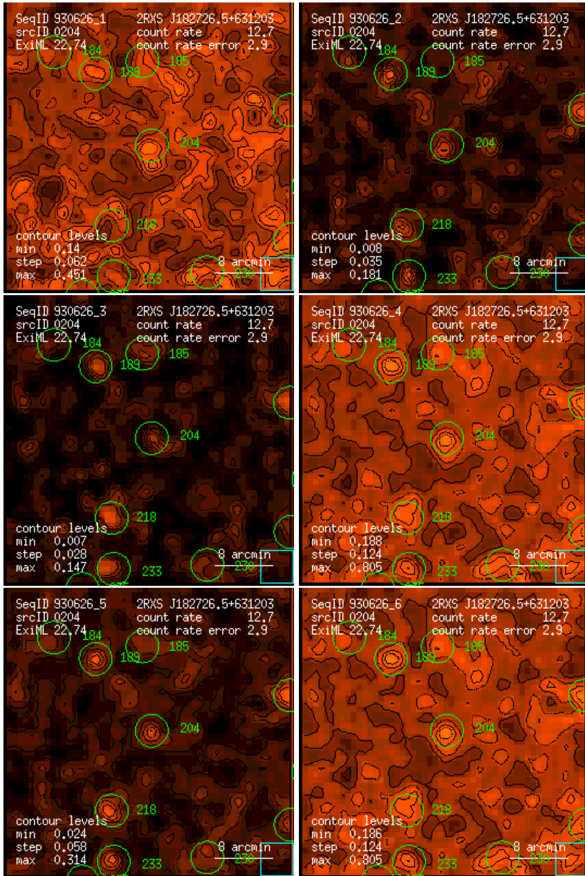
Figure 204: RASS 930626: detection 0204: band rate images, Gaussian filter: (1) PSPC channels 11 – 41, (2) 52 – 90, (3) 91 – 201, (4) 11 – 235, (5) 52 – 201, (6) 11 – 201. Broad band rates in counts/ks. Band rate contour levels in counts/ks/arcmin 2 .
