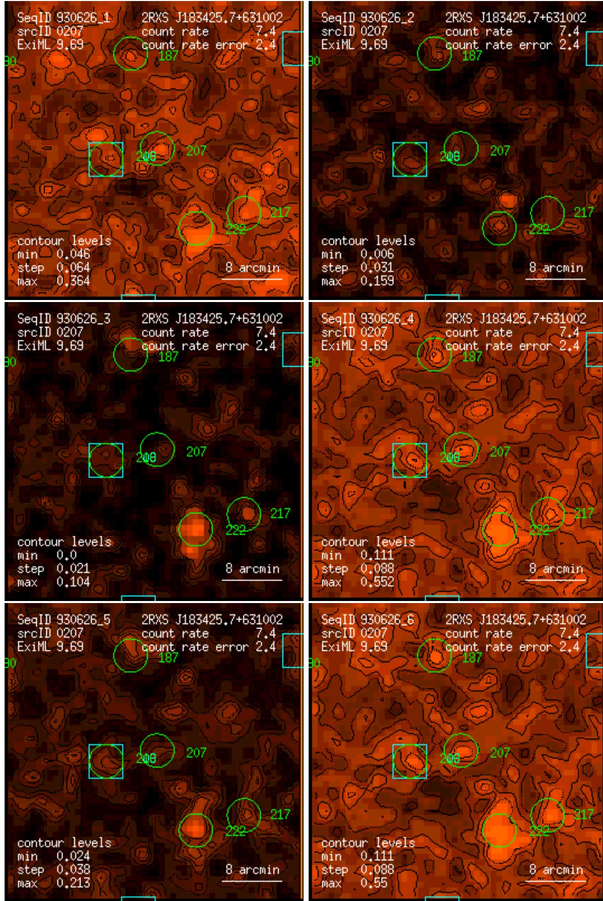
Figure 207: RASS 930626: detection 0207: band rate images, Gaussian filter: (1) PSPC channels 11 – 41, (2) 52 – 90, (3) 91 – 201, (4) 11 – 235, (5) 52 – 201, (6) 11 – 201. Broad band rates in counts/ks. Band rate contour levels in counts/ks/arcmin 2 .
