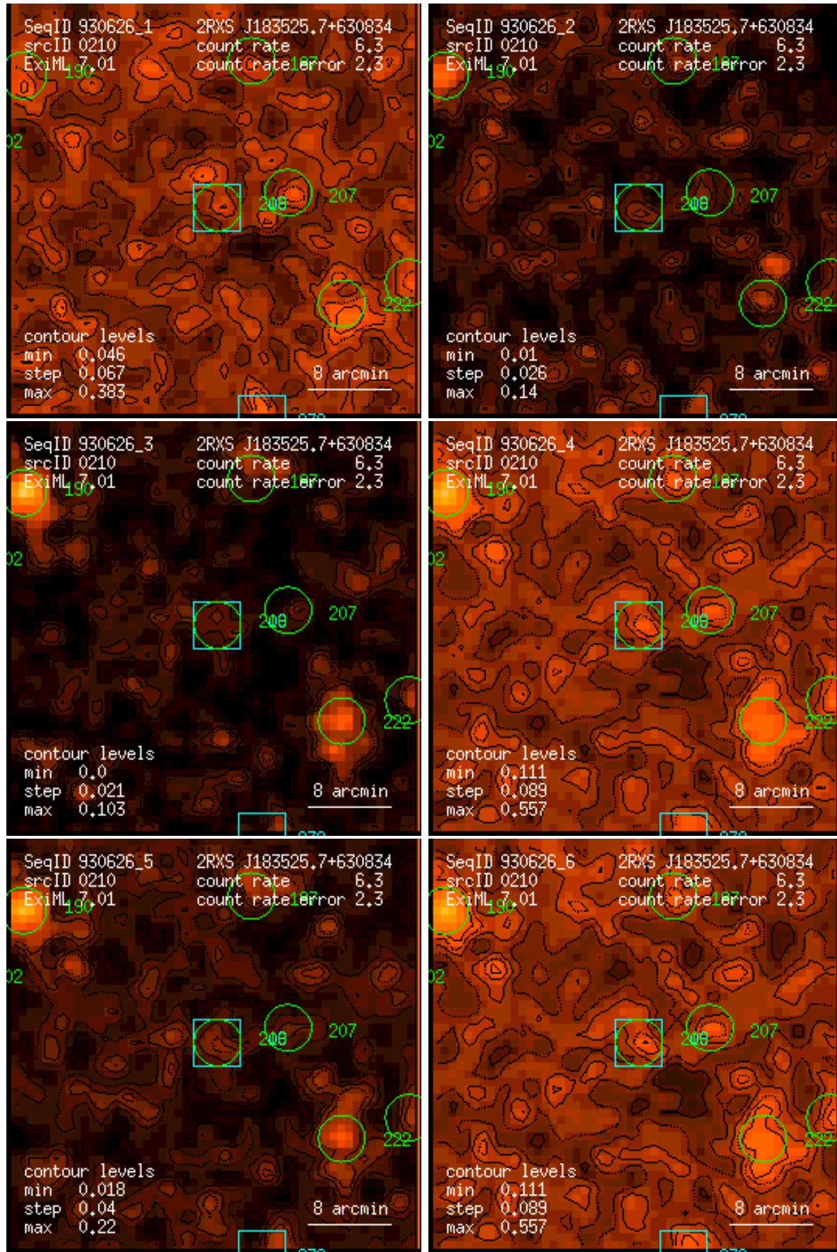
Figure 210: RASS 930626: detection 0210: band rate images, Gaussian filter: (1) PSPC channels 11 – 41, (2) 52 – 90, (3) 91 – 201, (4) 11 – 235, (5) 52 – 201, (6) 11 – 201. Broad band rates in counts/ks. Band rate contour levels in counts/ks/arcmin 2 .
