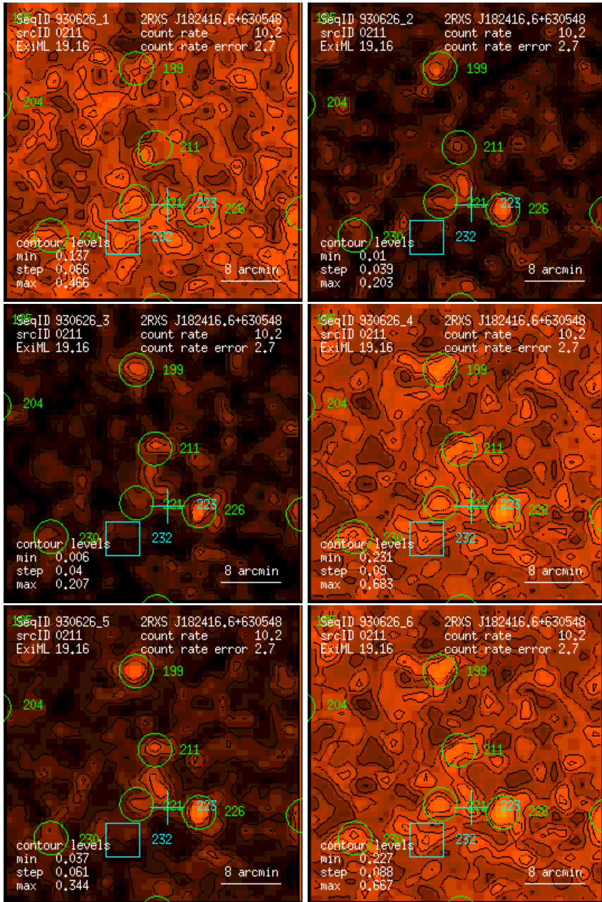
Figure 211: RASS 930626: detection 0211: band rate images, Gaussian filter: (1) PSPC channels 11 – 41, (2) 52 – 90, (3) 91 – 201, (4) 11 – 235, (5) 52 – 201, (6) 11 – 201. Broad band rates in counts/ks. Band rate contour levels in counts/ks/arcmin 2 .
